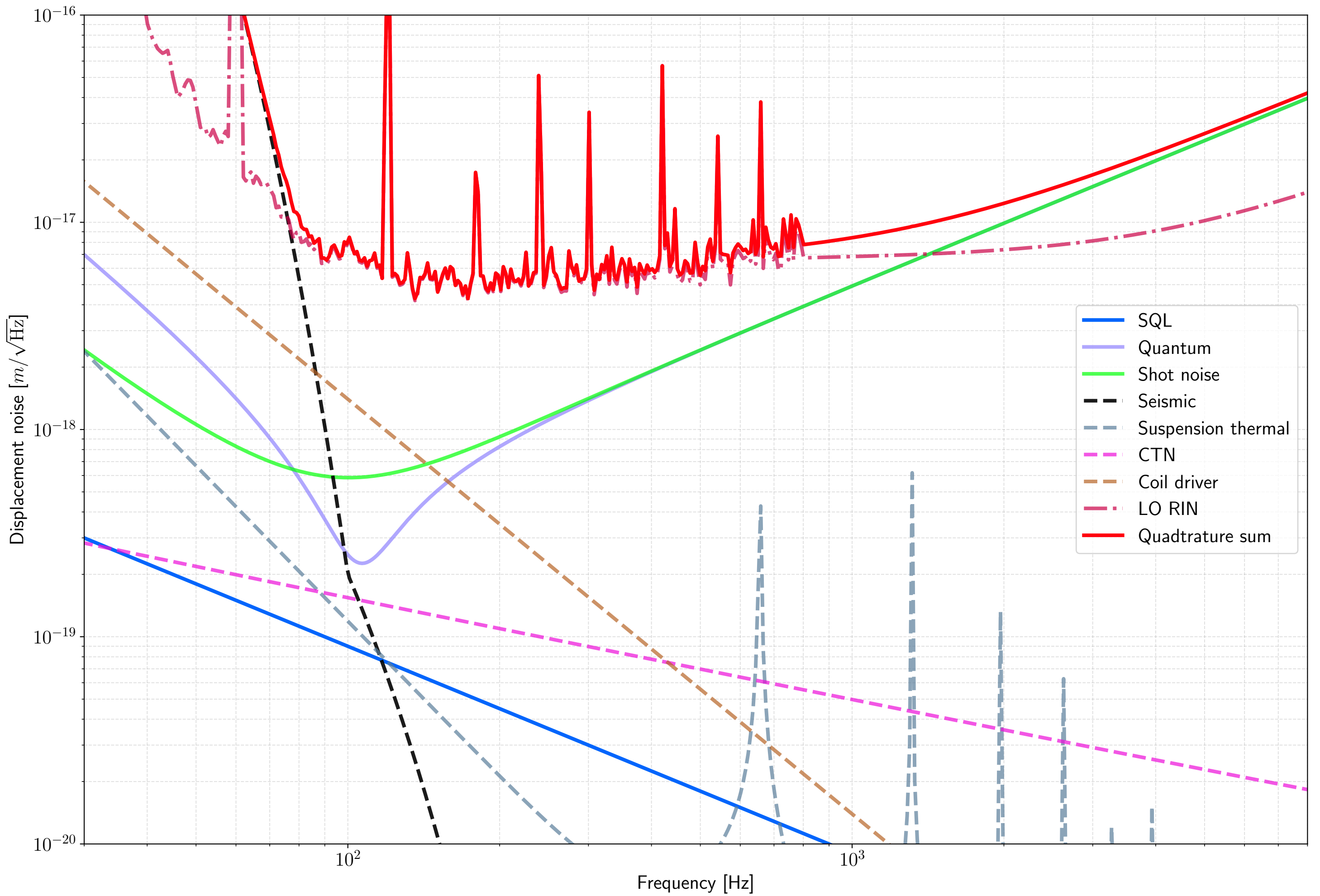
Analytic noise budget for 40m Ponderomotive Squeezing experiment
