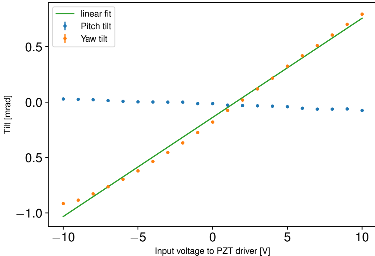
2inch PZT Mirror Calibration - Input to PZT Yaw (CH1)
