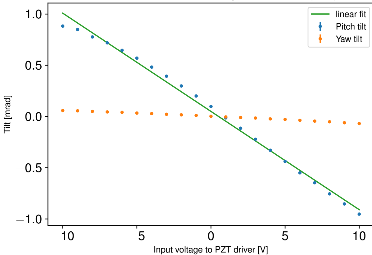
2inch PZT Mirror Calibration - Input to PZT Pitch (CH2)
