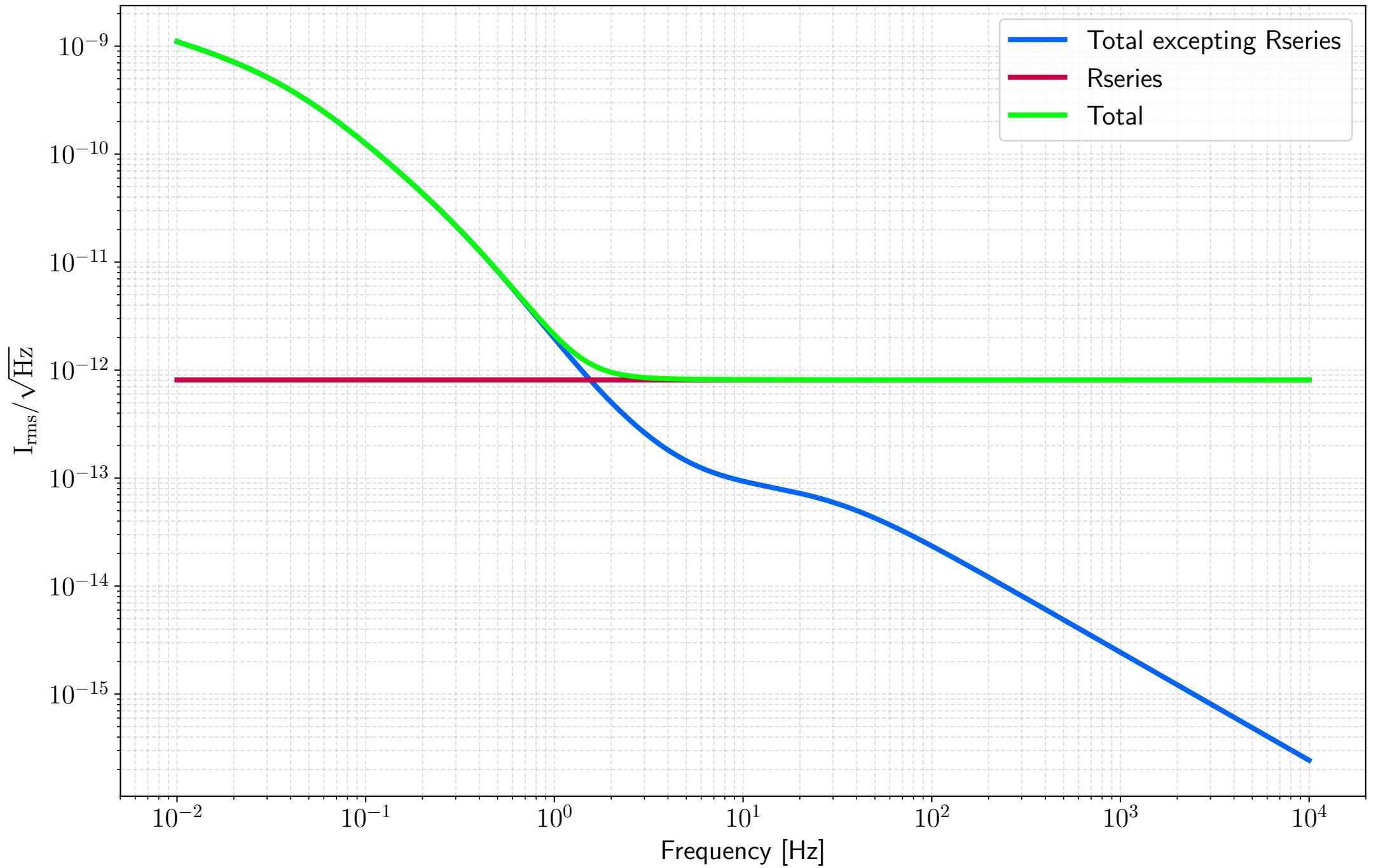
Current noise of Coil Driver HV bias path
