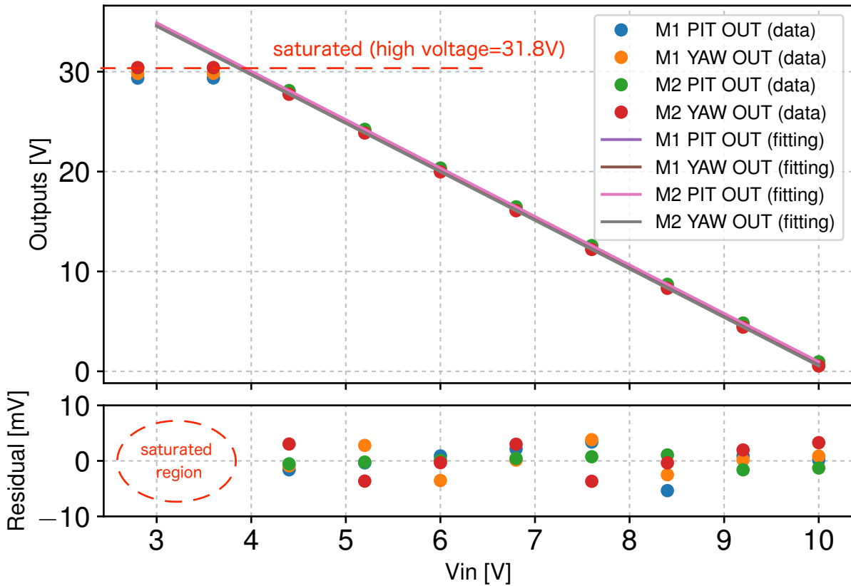
PZT driver performance (OUT)
