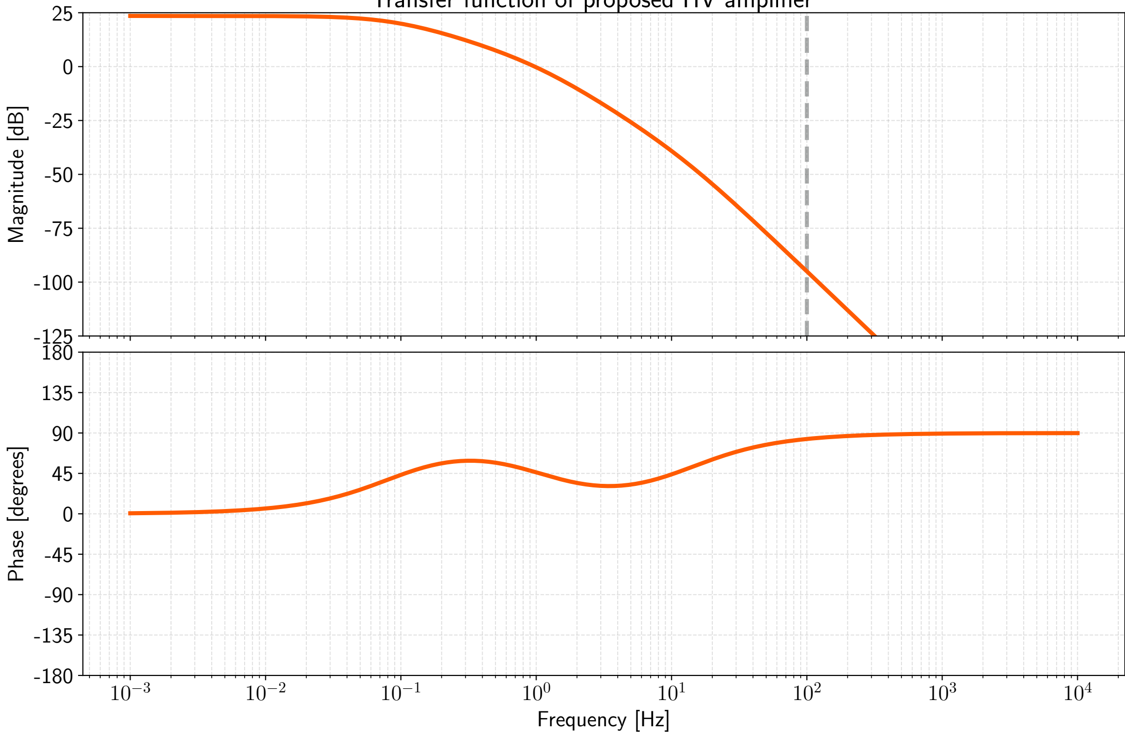
Transfer function of proposed HV amplifier
