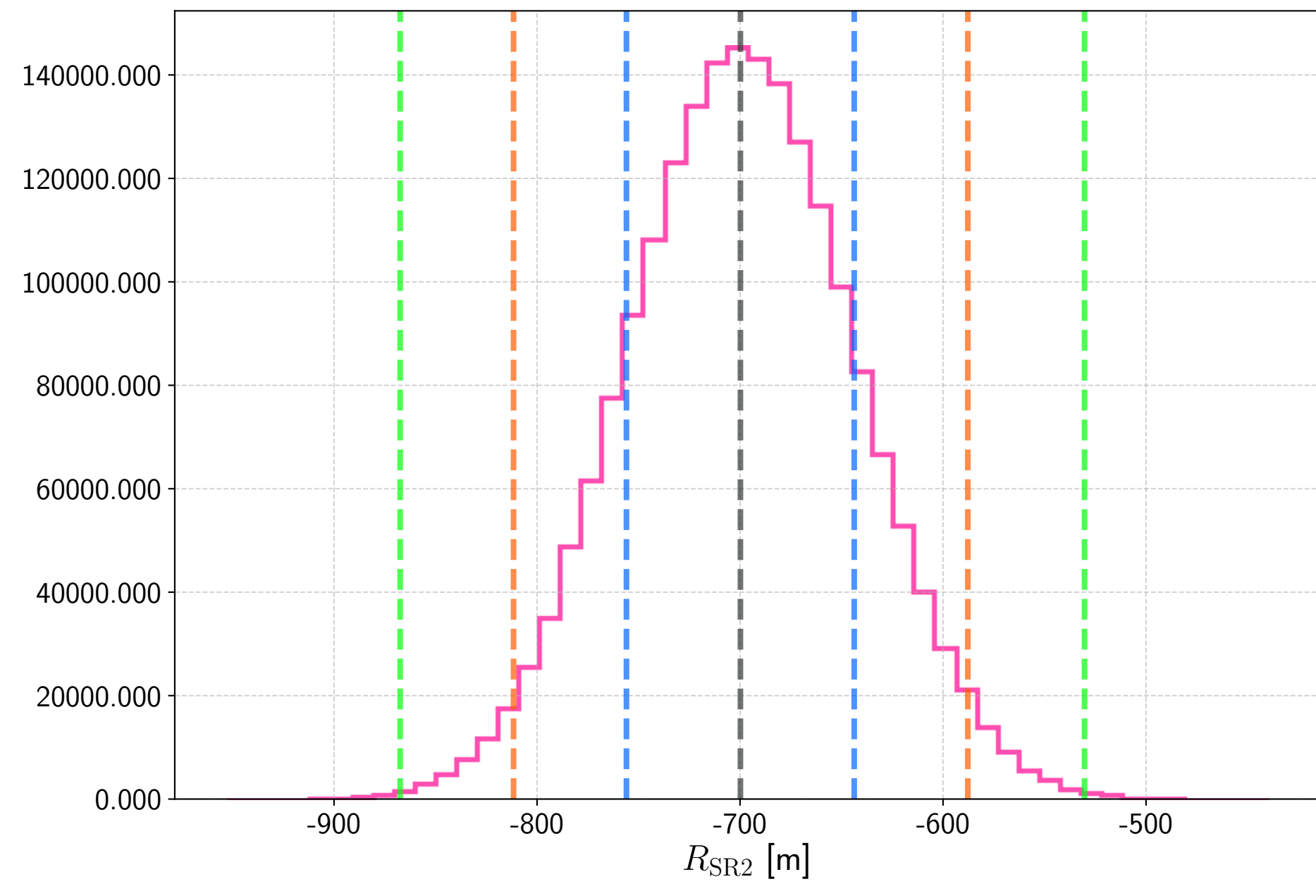
Histograms of perturbations used to generate corner plot for SRC
