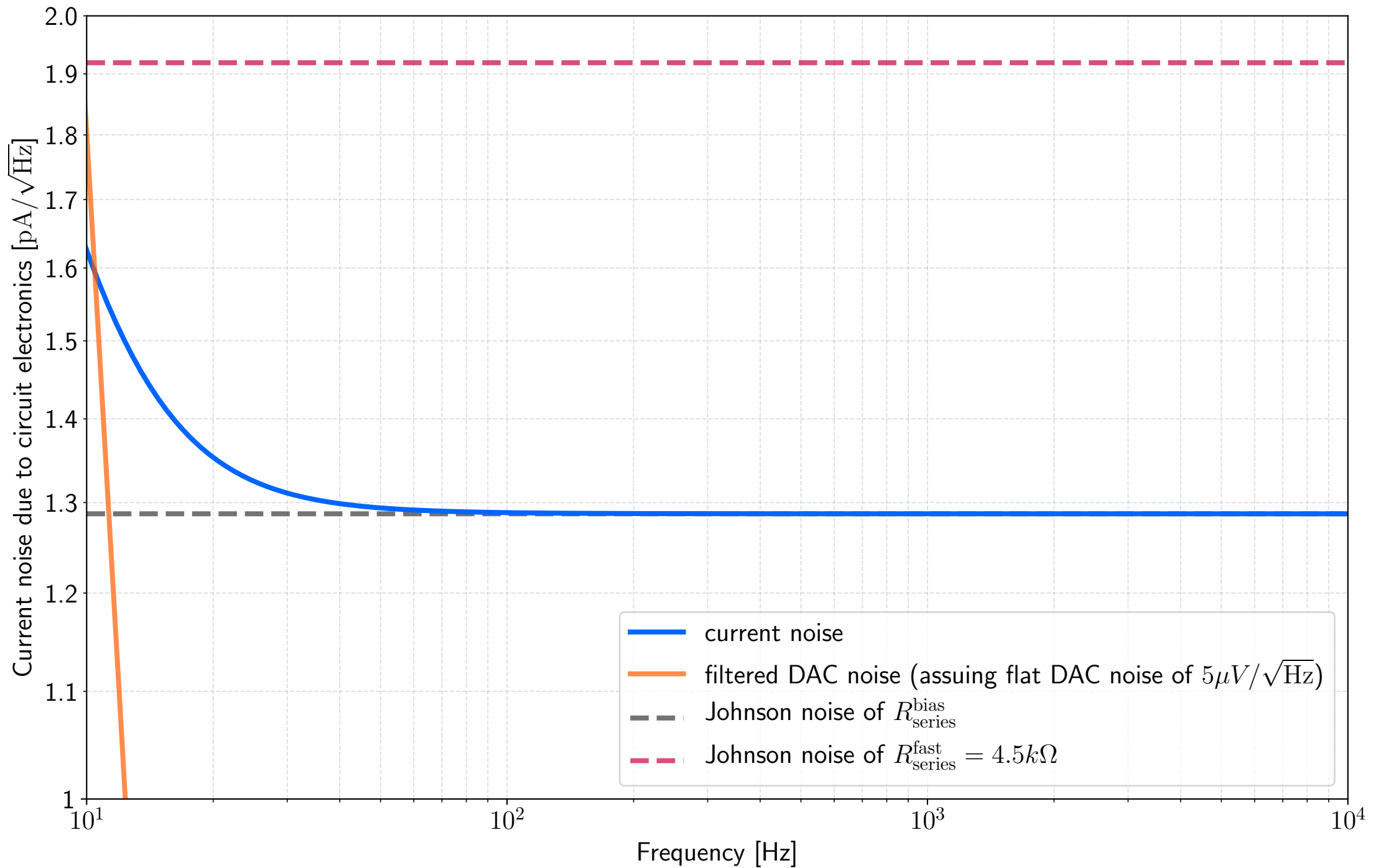
HV bias path current noise for R_{\text{series}}^{\text{bias}} = 10.0 \text{ k}\Omega
