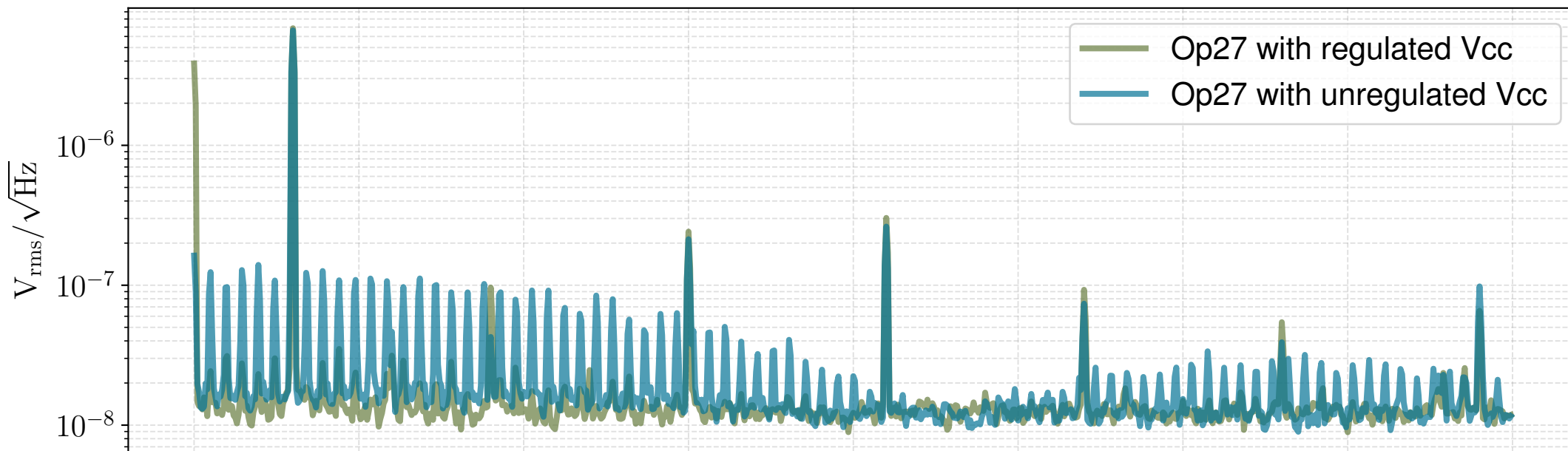
PSRR of Op27 (120dB typ) and LT1128 (132dB typ)
