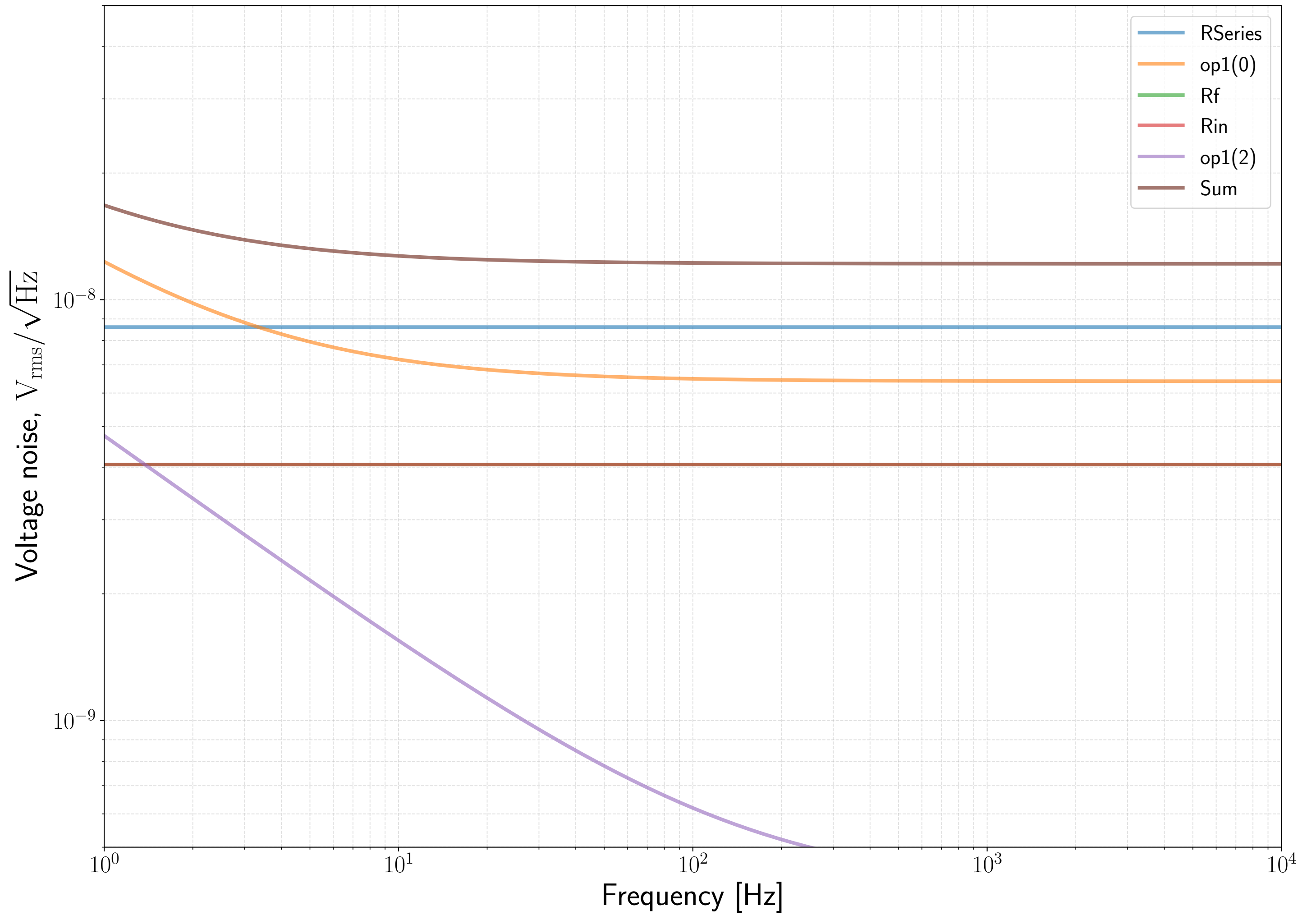
D010001 ETMX Coil Driver Noises (Fast path only), R_{\text{series}} = 4.5\text{k}\Omega
