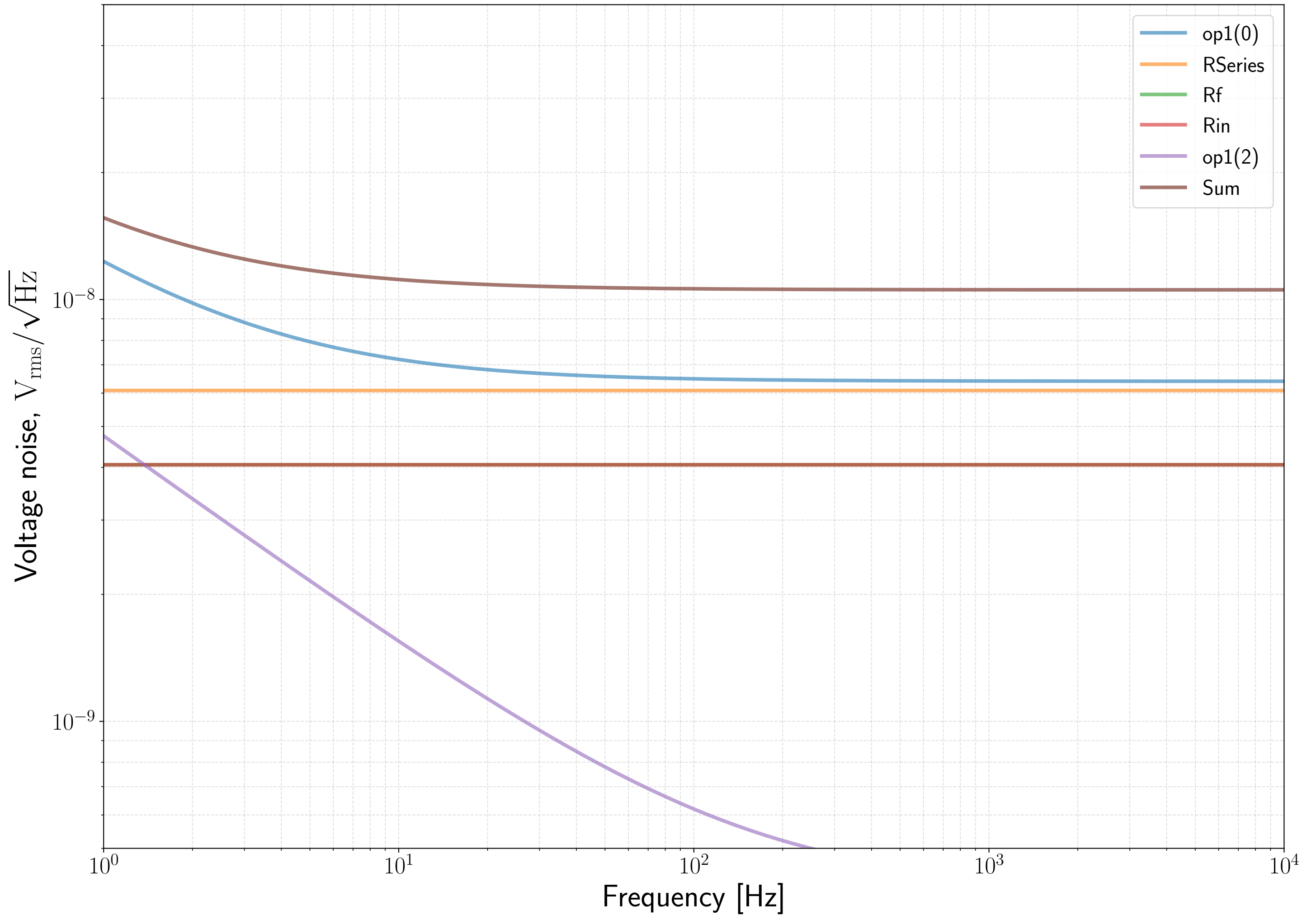
D010001 ETMX Coil Driver Noises (Fast path only), R_{\text{series}} = 2.25\text{k}\Omega
