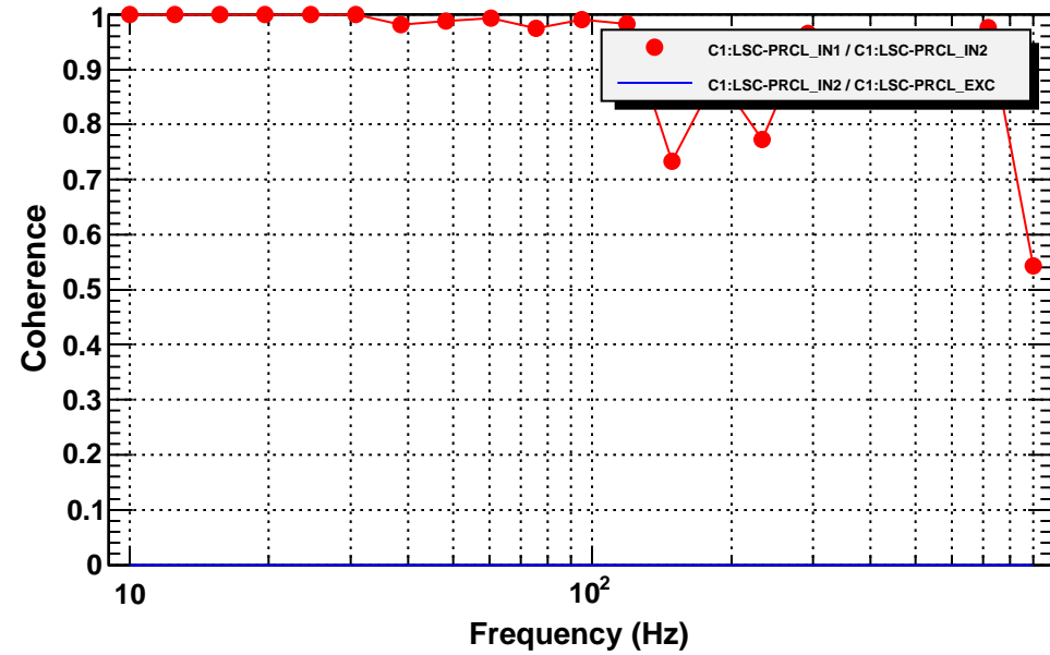
PRCL Coherence function
