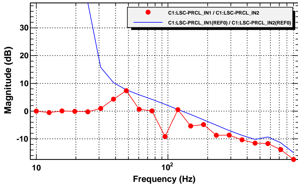
PRCL Open Loop Gain
