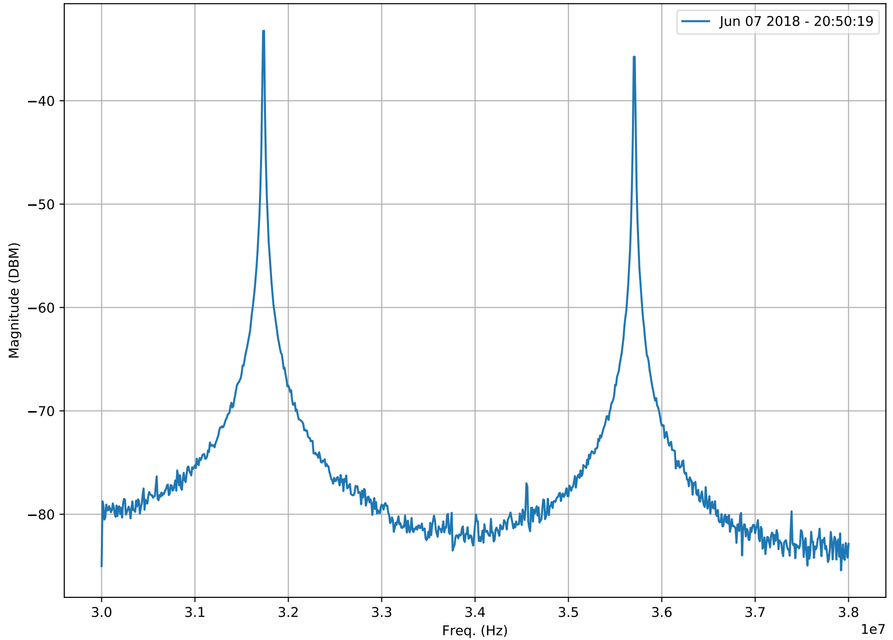
AG4395A Spectrum - Jun 07 2018 - 20:50:36
