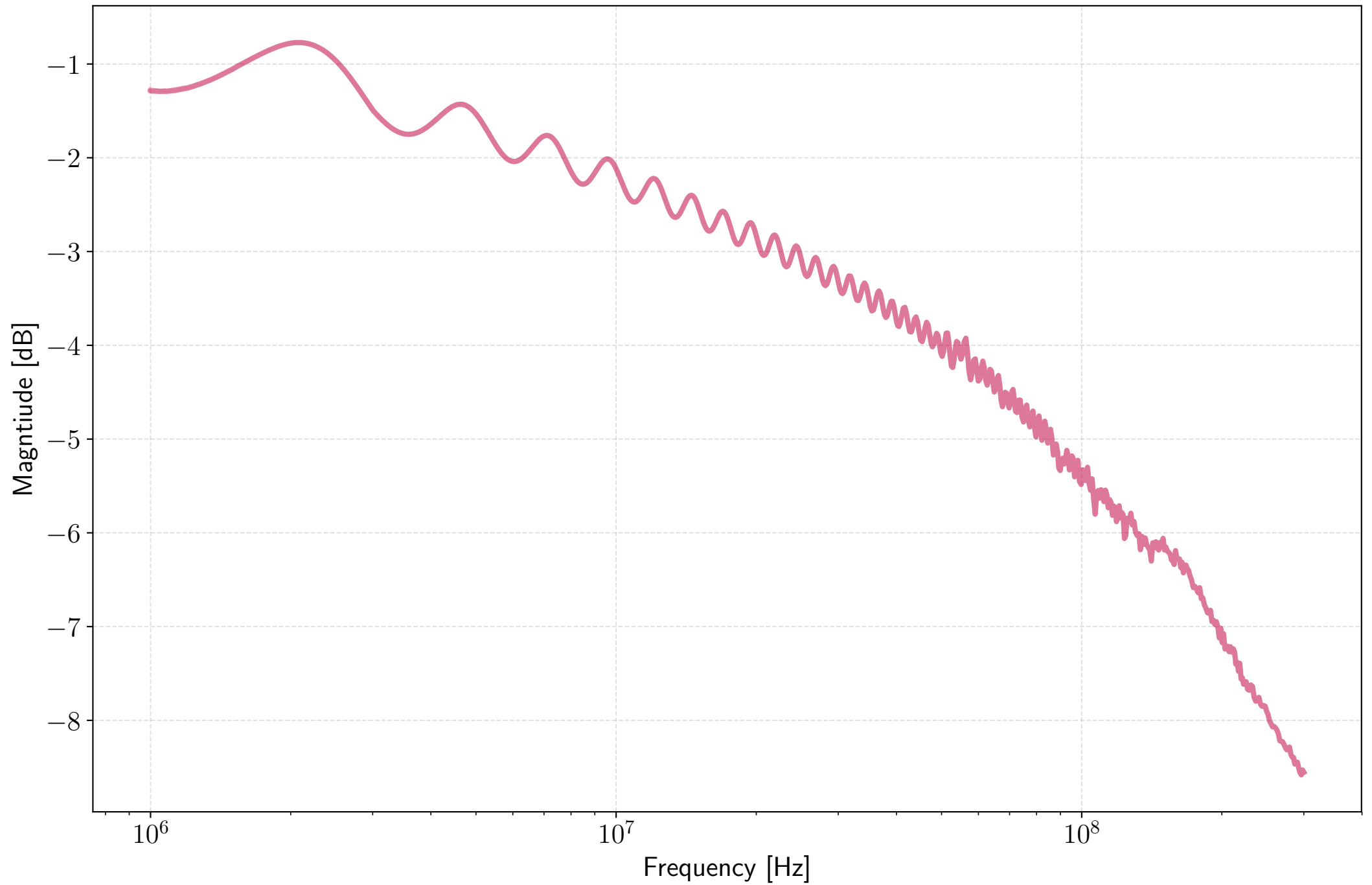
Delay line TF magnitude (X arm)
