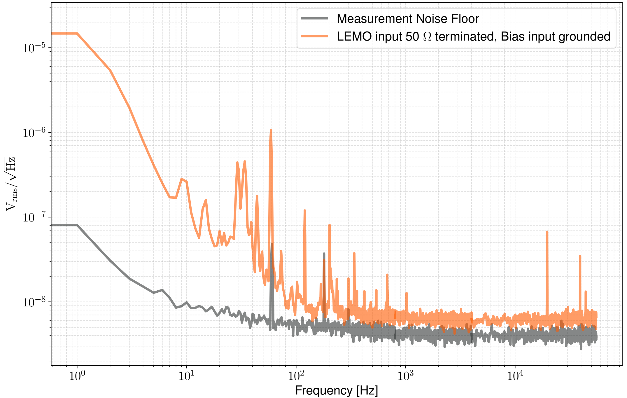
MC1 coil driver UL channel electronics noise (measured in office area)
