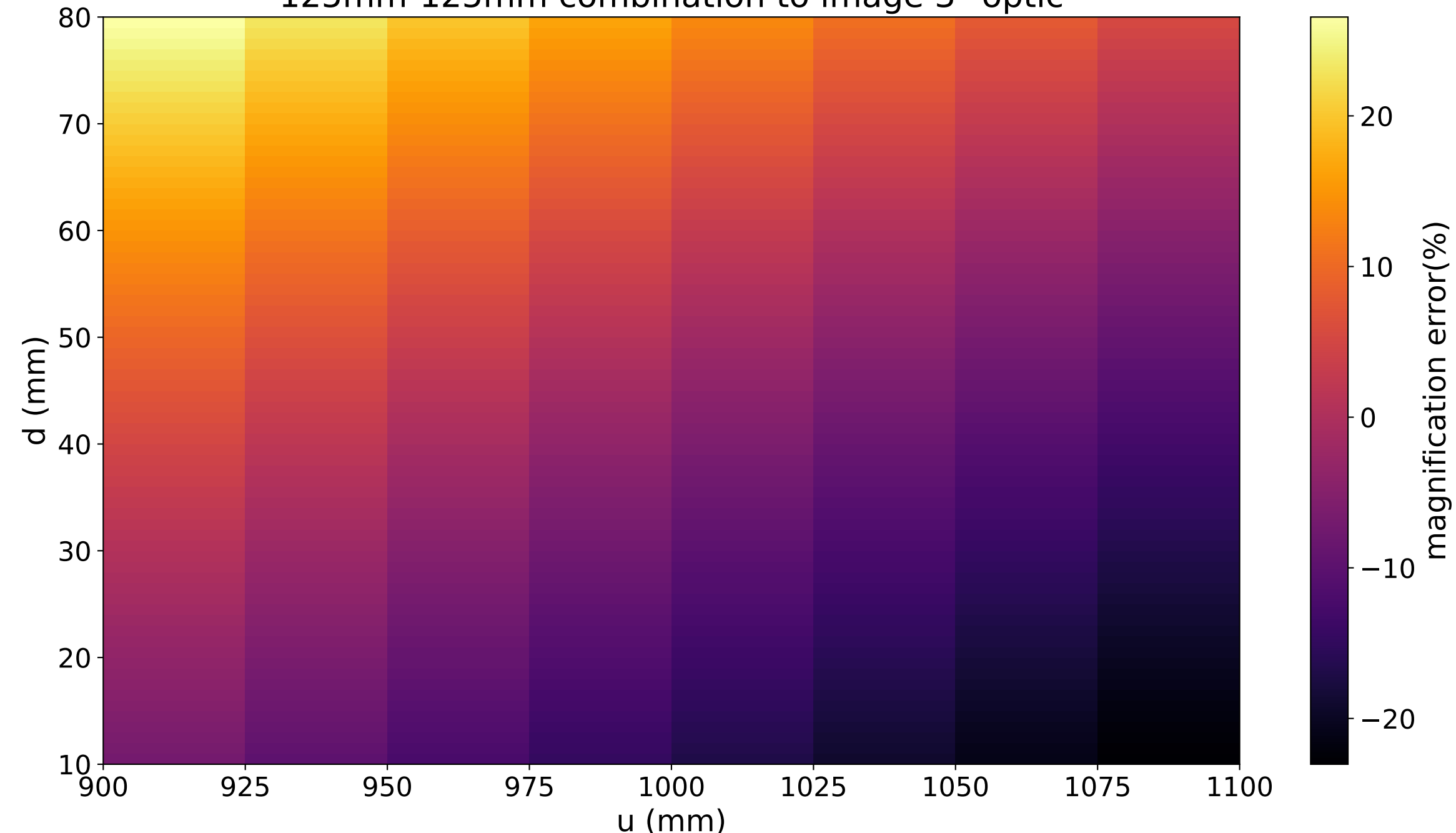
125mm-125mm combination to image 3" optic
