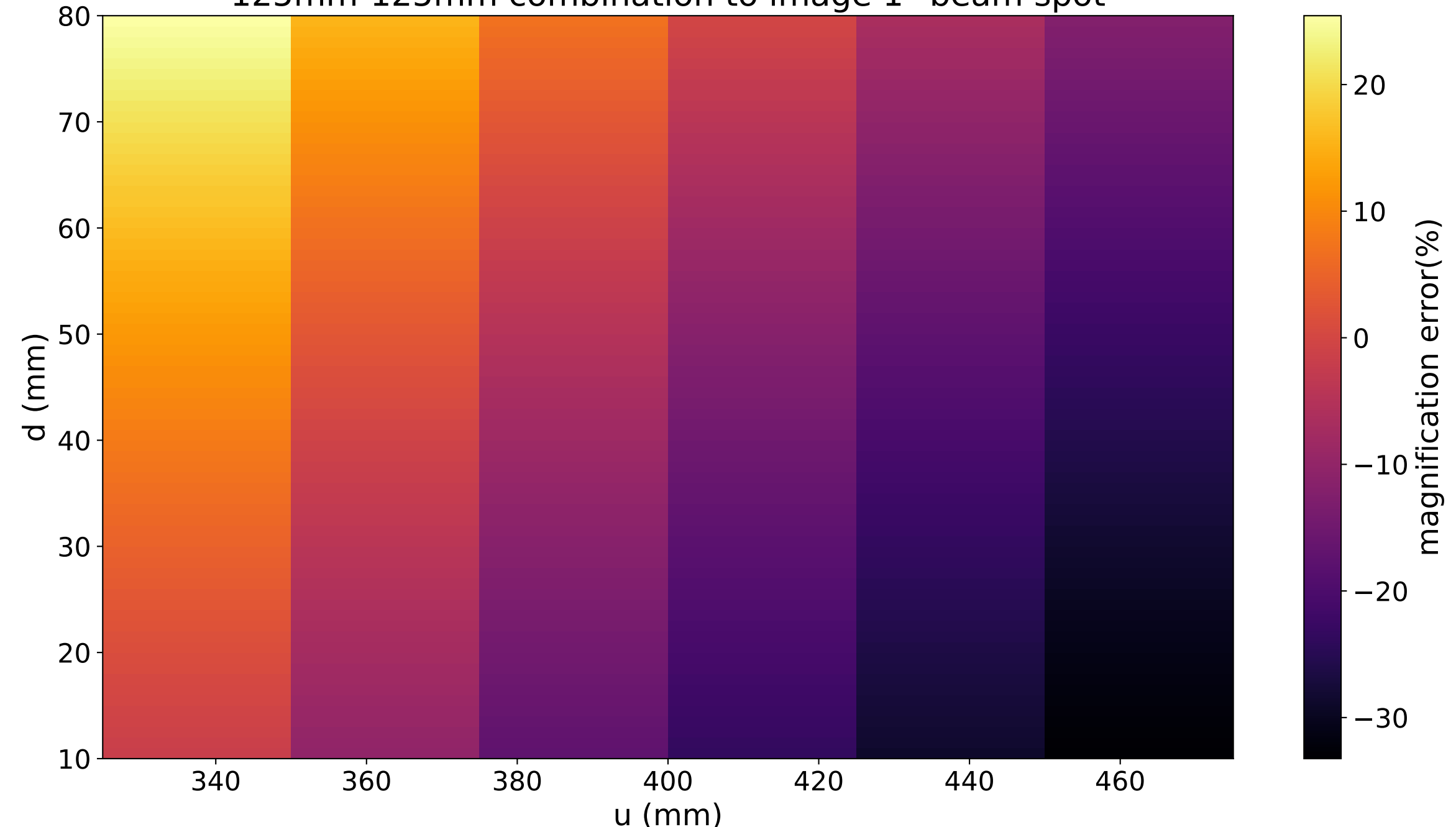
125mm-125mm combination to image 1" beam spot
