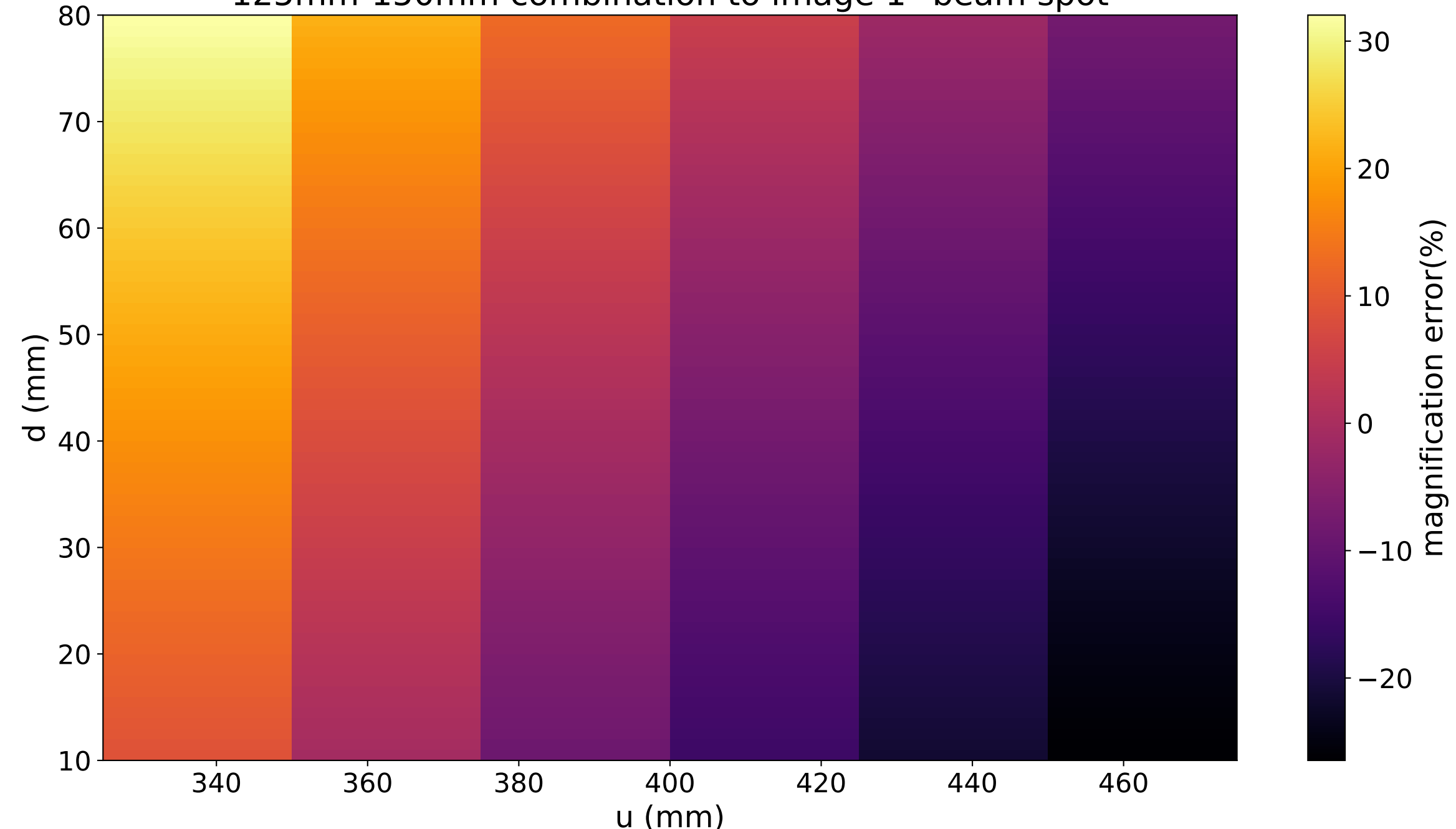
125mm-150mm combination to image 1" beam spot
