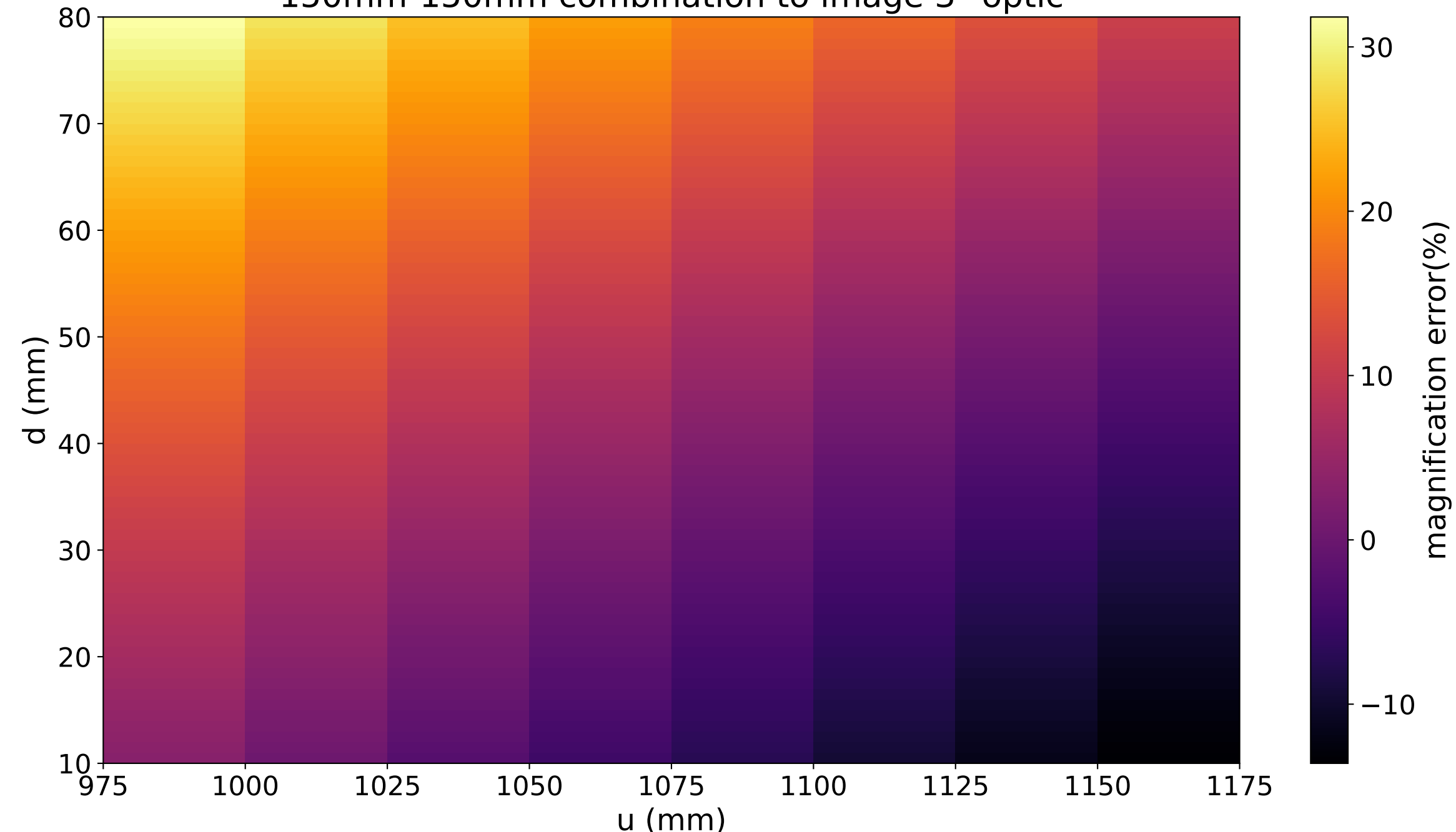
150mm-150mm combination to image 3" optic
