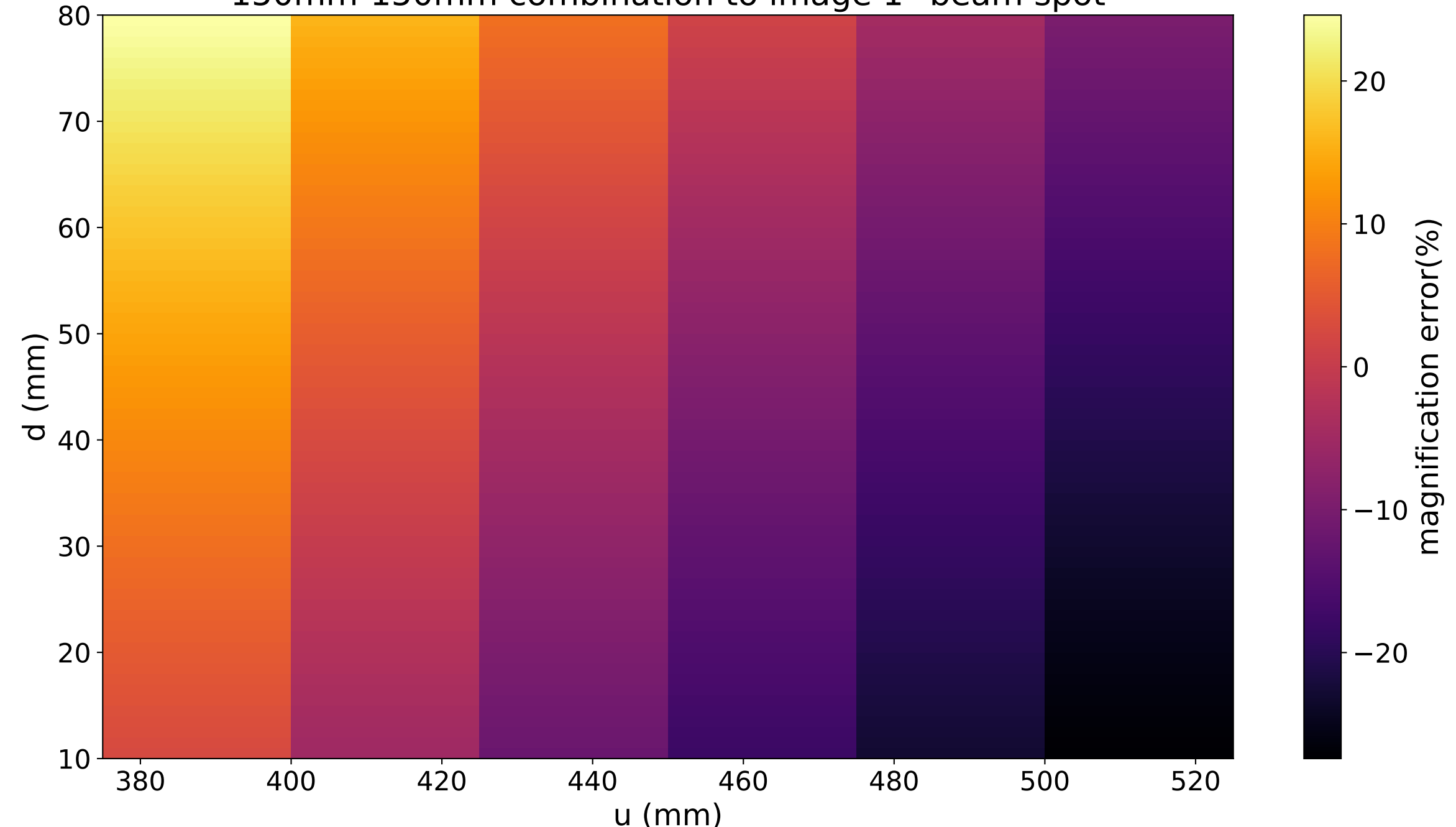
150mm-150mm combination to image 1" beam spot
