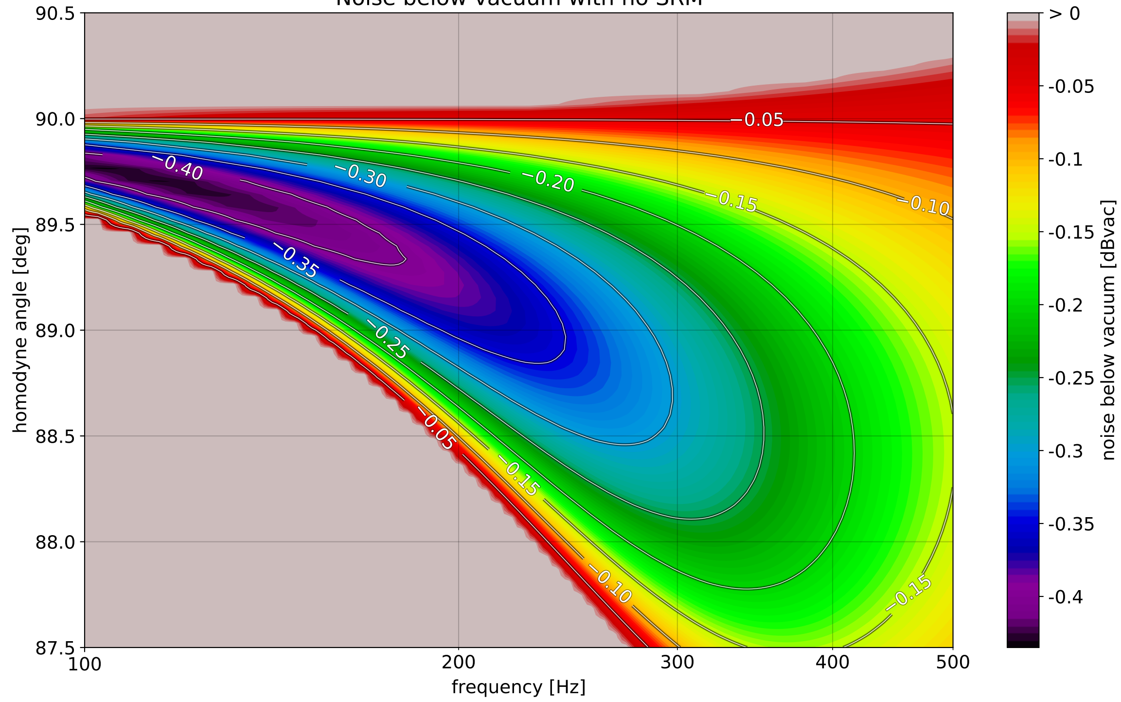
Noise below vacuum with no SRM
