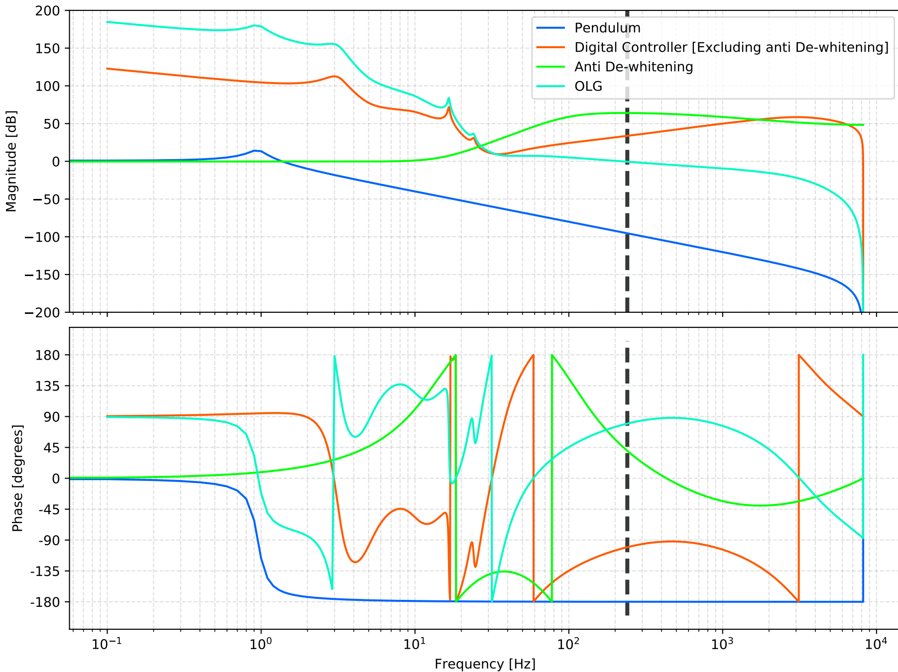
DARM OLF assuming 2015 October DRFPMI locking loop shape
