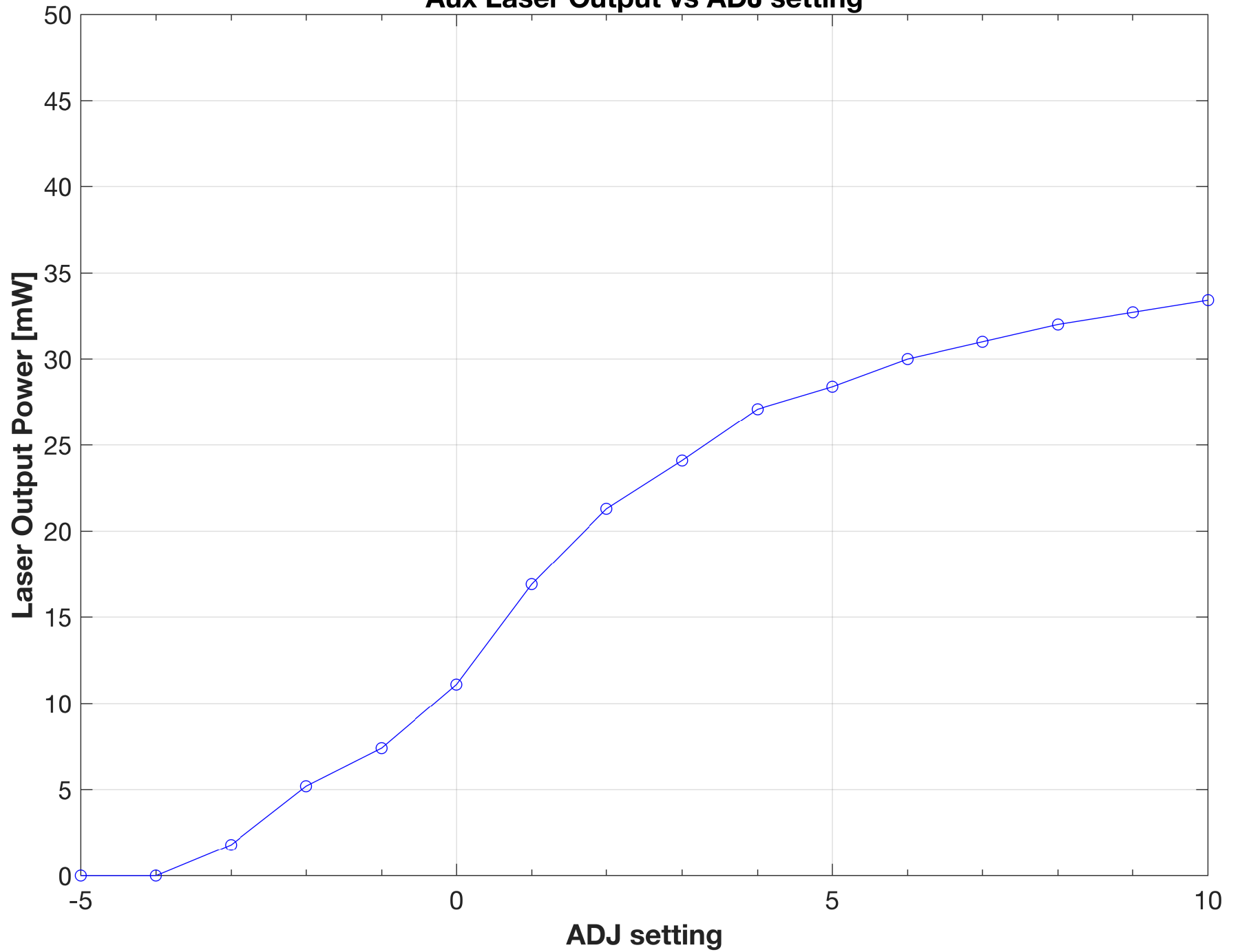
Aux Laser Output vs ADJ setting
