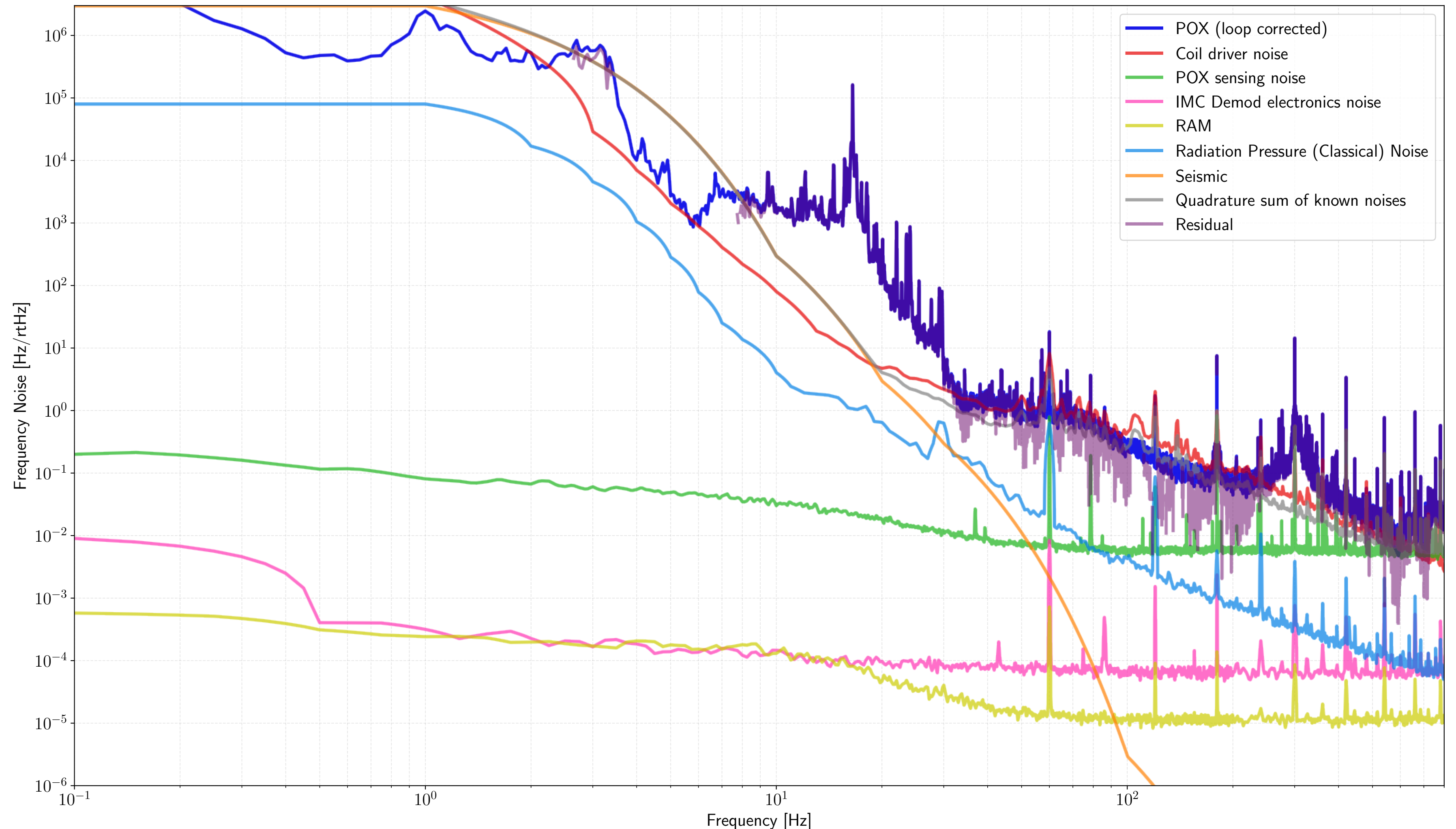
40m IMC Noise Budget
