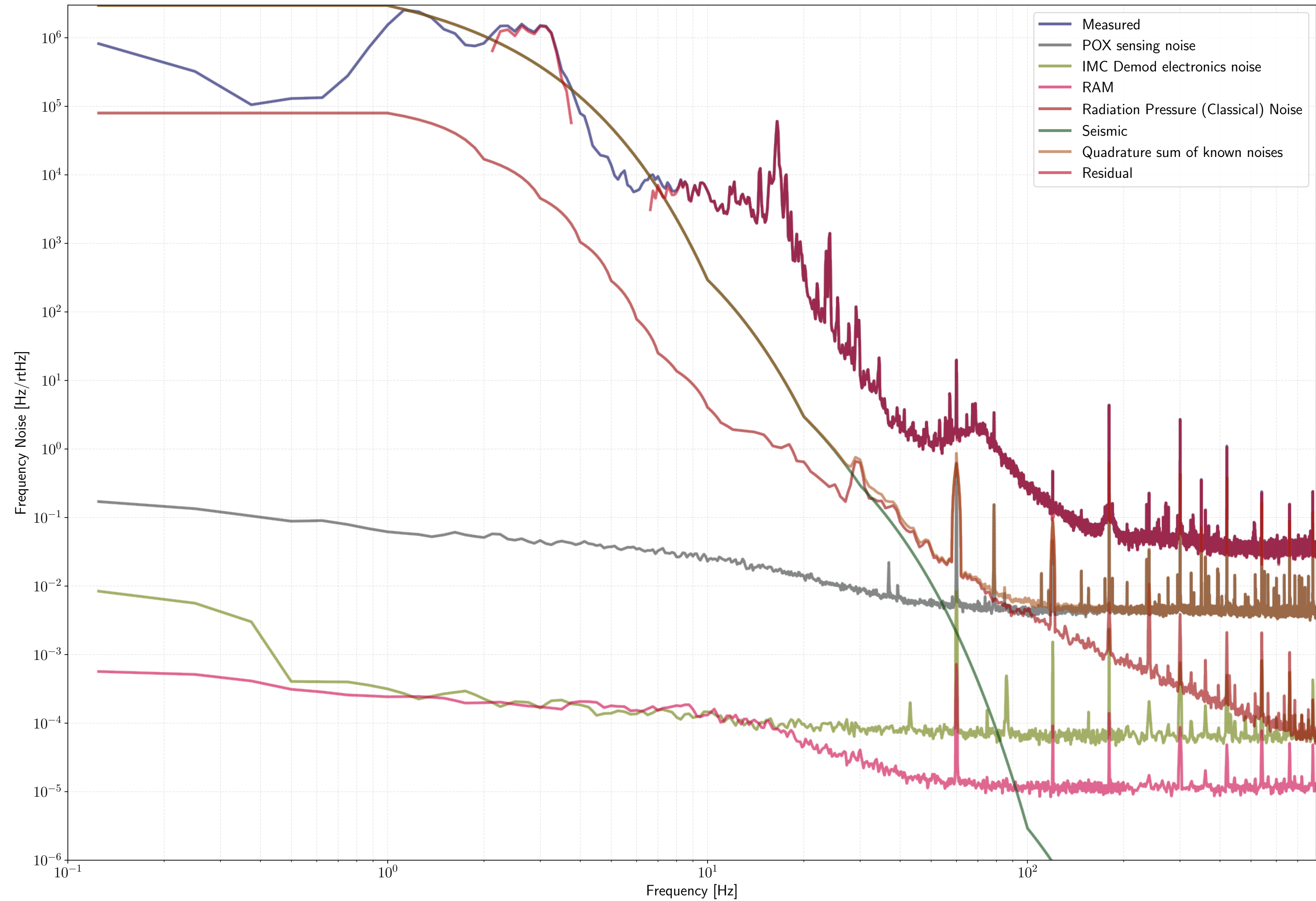
40m IMC Noise Budget
