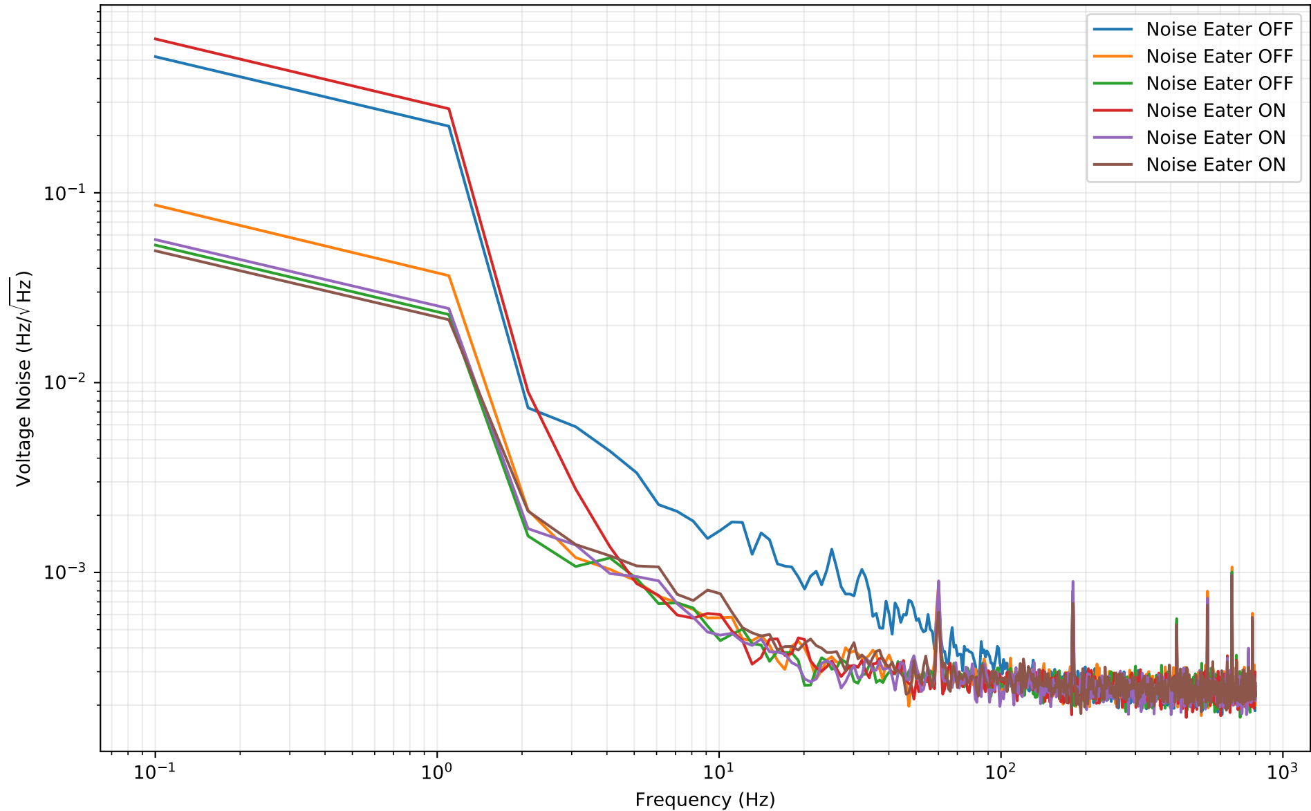
MCREFLPD Noise Eater Measurement
