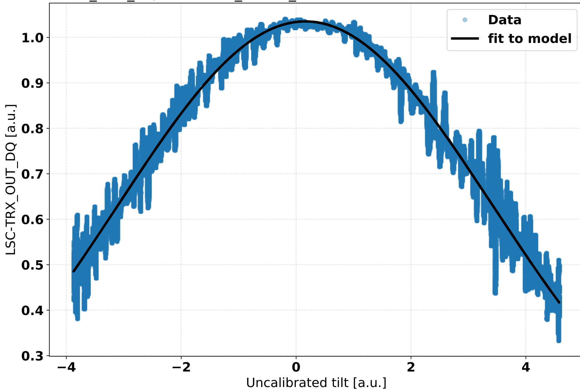
LSC-TRX_OUT_DQ vs SUS-BS_OPLEV_YERROR from 1194920533 to 1194920600
