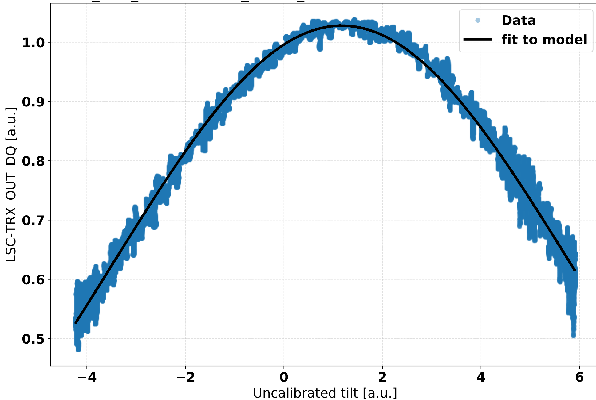
LSC-TRX_OUT_DQ vs SUS-BS_OPLEV_PERROR from 1194919884 to 1194919950
