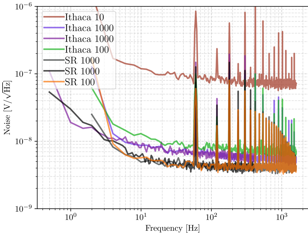
Input referred noise of the Ithaca 1201 preamp
