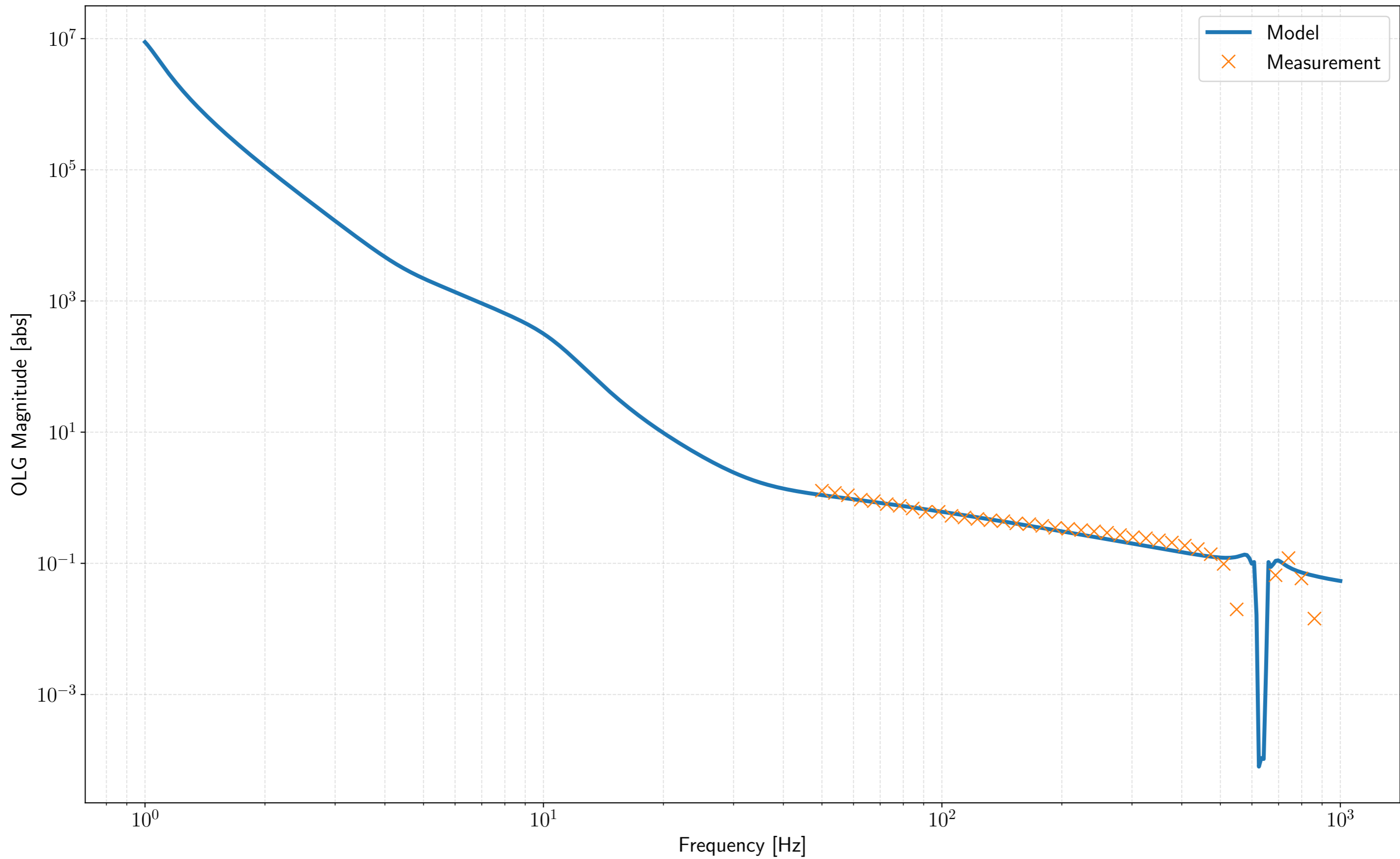
MICH measured vs modelled OLTF
