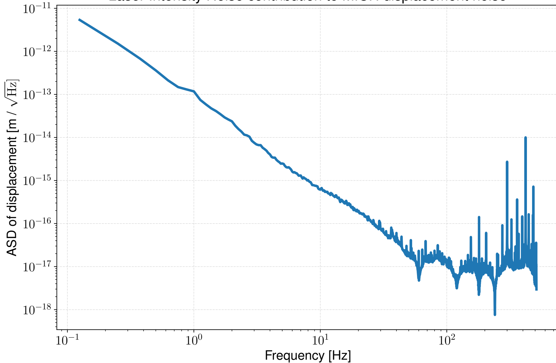
Laser Intensity Noise contribution to MICH displacement noise
