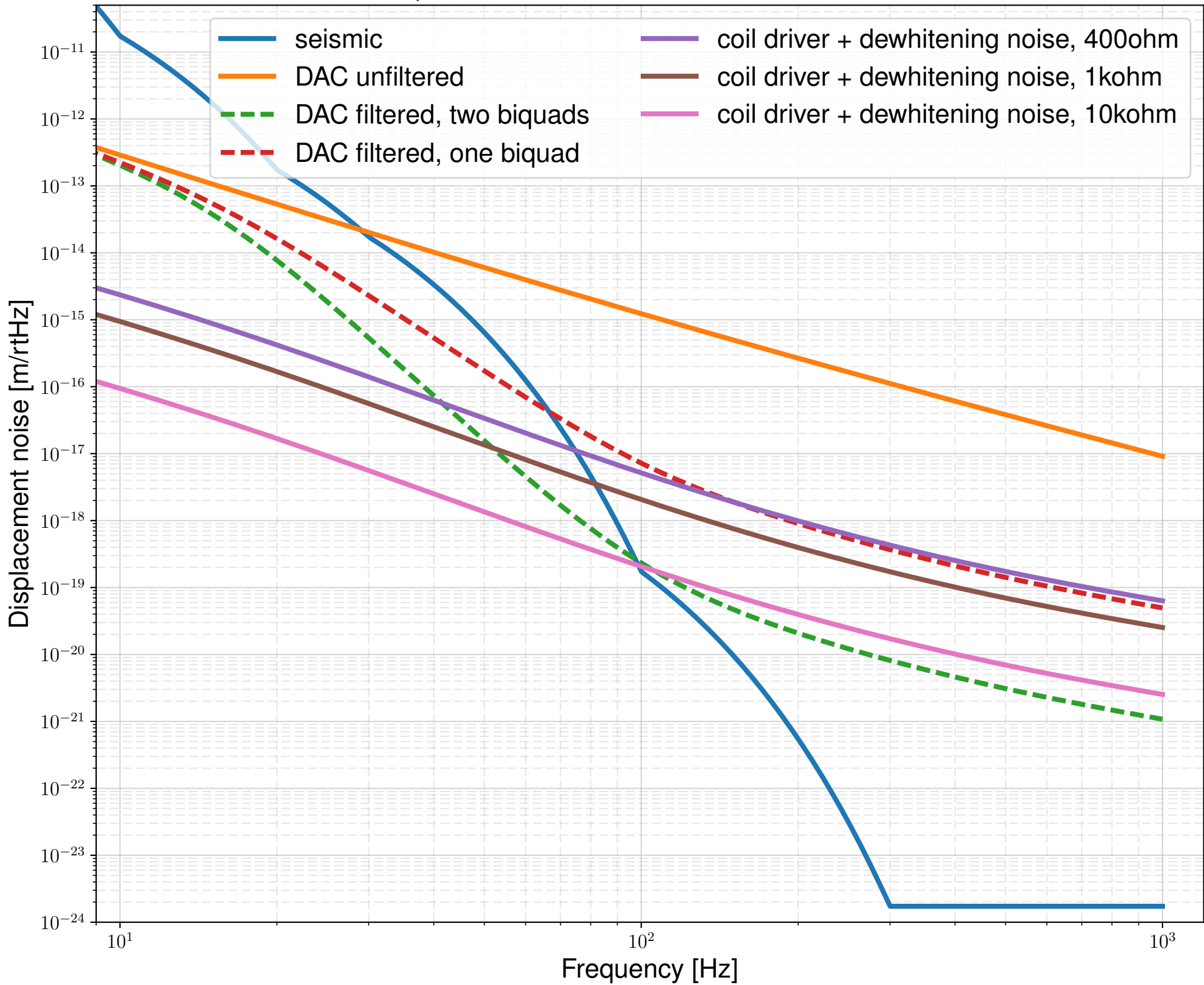
Comparison of seismic noise and coil-driver noise
