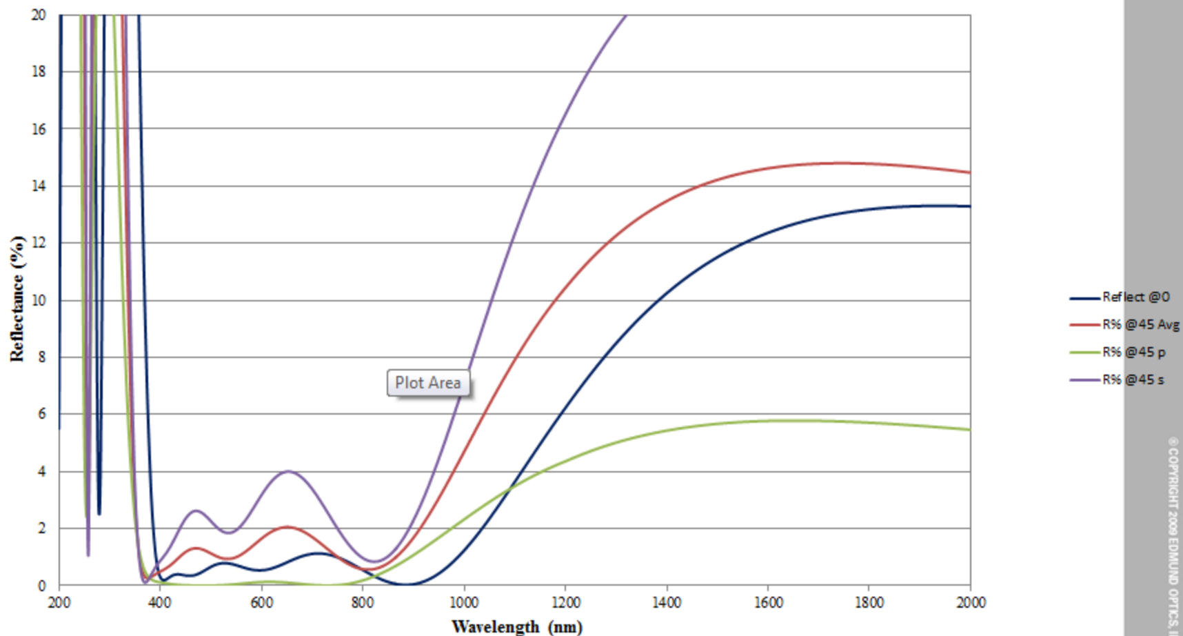
VIS-NIR 0 and 45 degree 200-2000nm FOR REFERENCE ONLY
