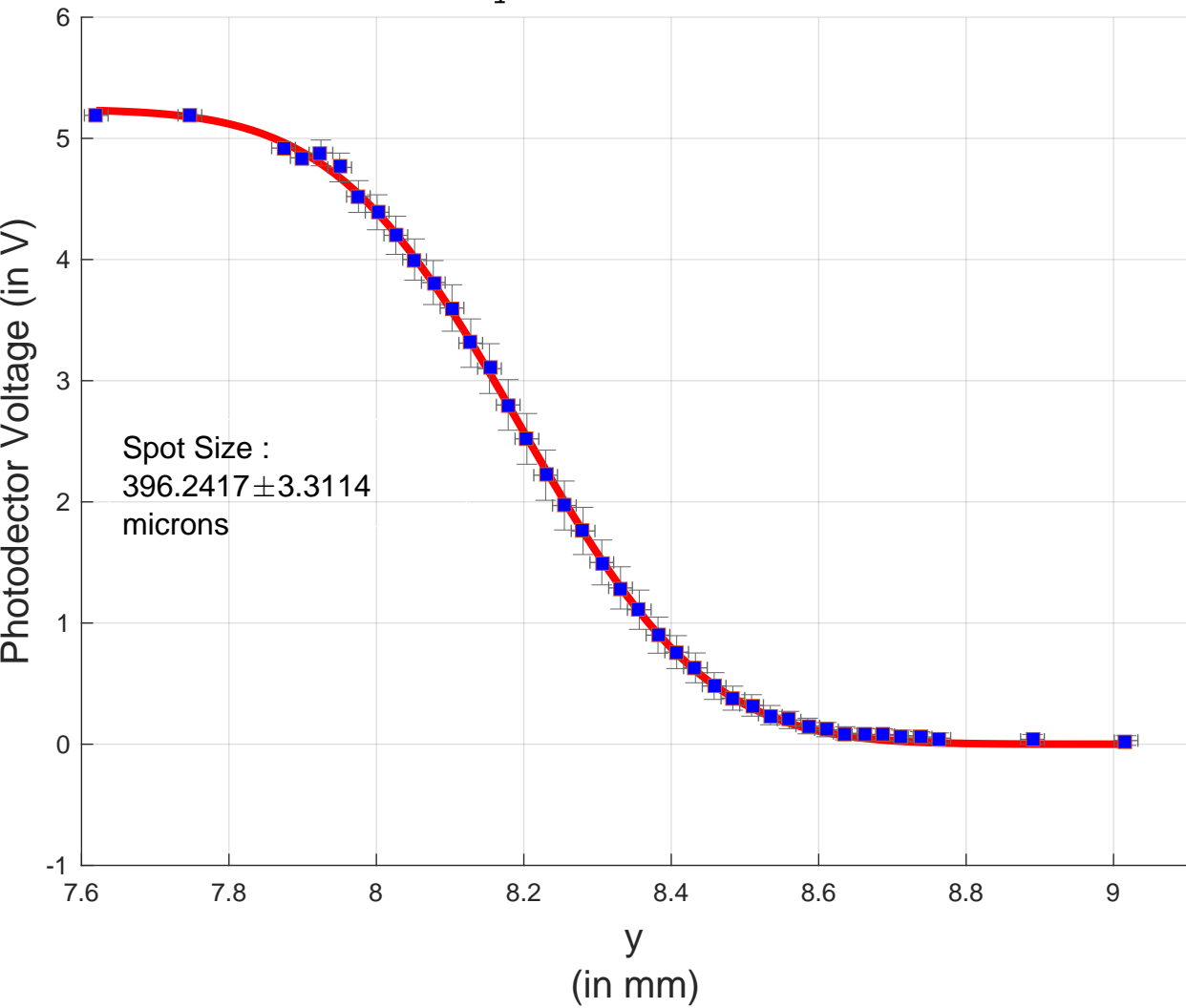
Beam y-Profile at z =35 cm
