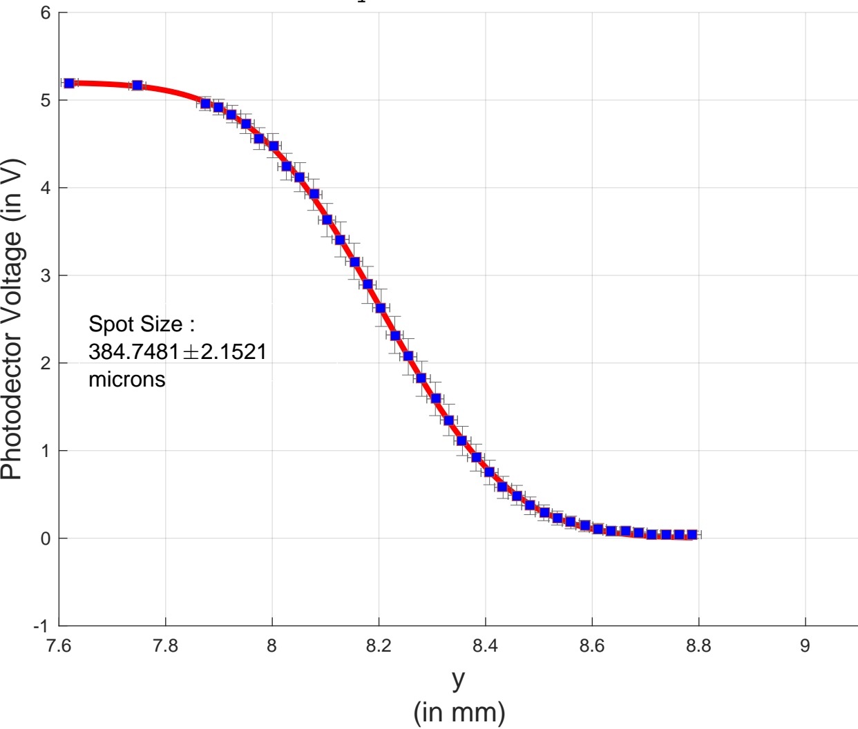
Beam y-Profile at z =30 cm
