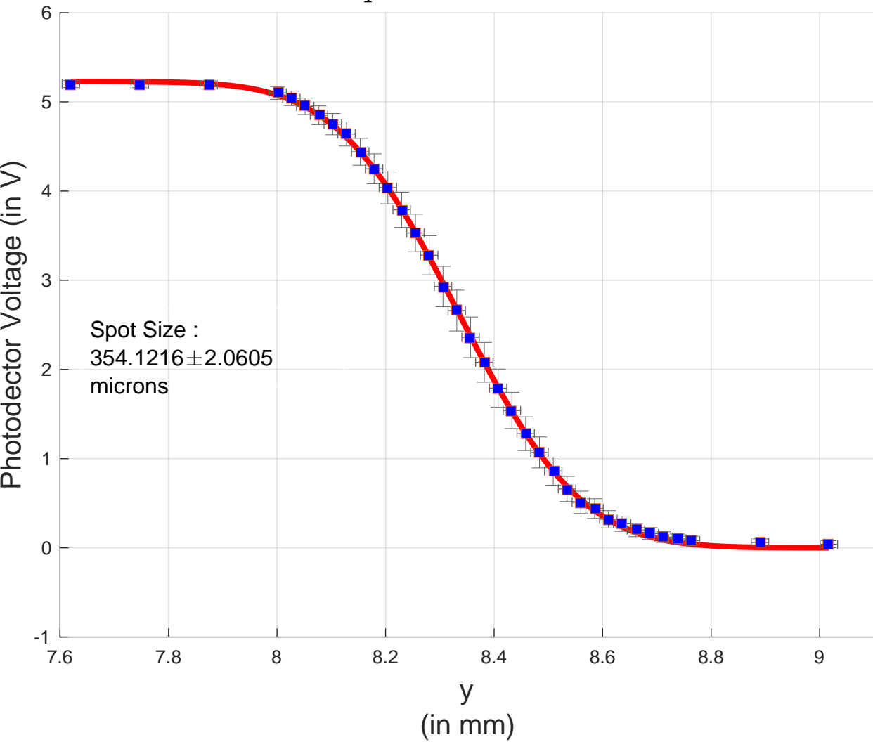
Beam y-Profile at z =20 cm
