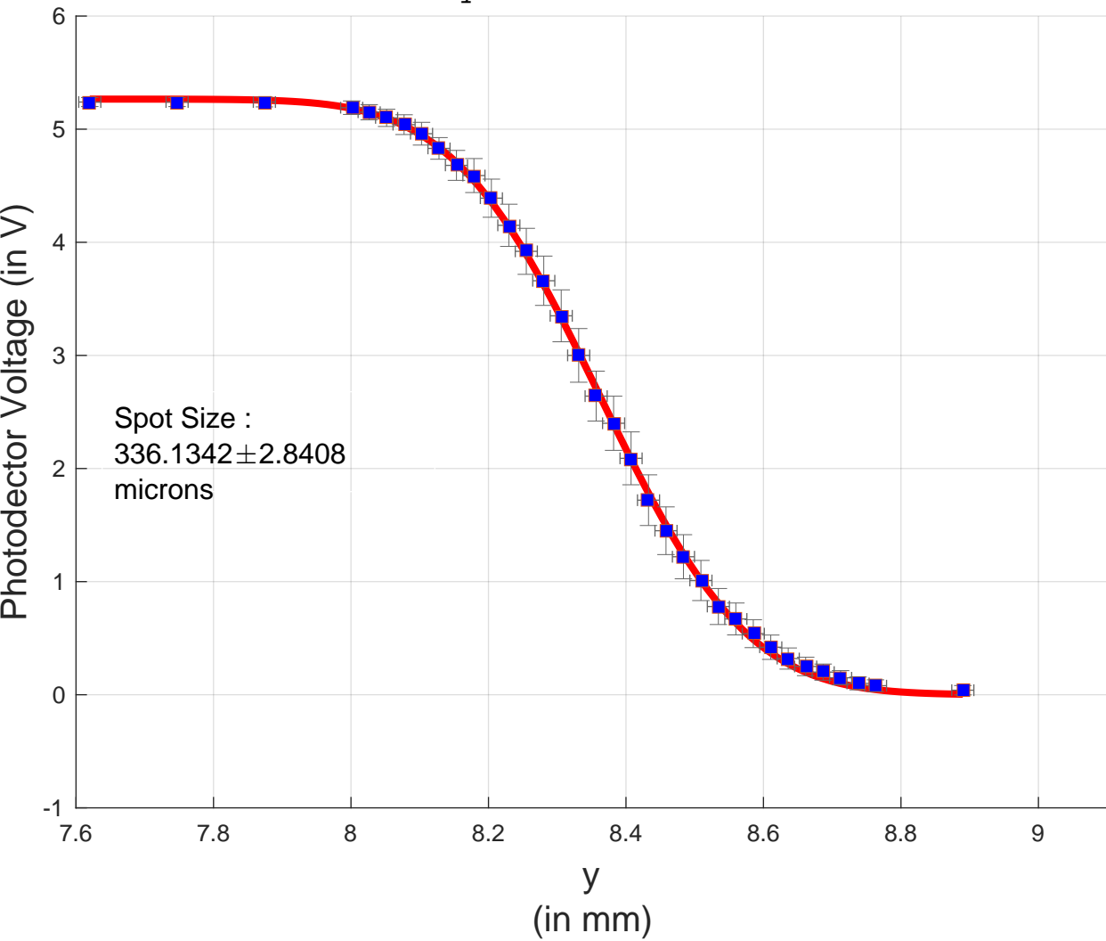
Beam y-Profile at z =10 cm
