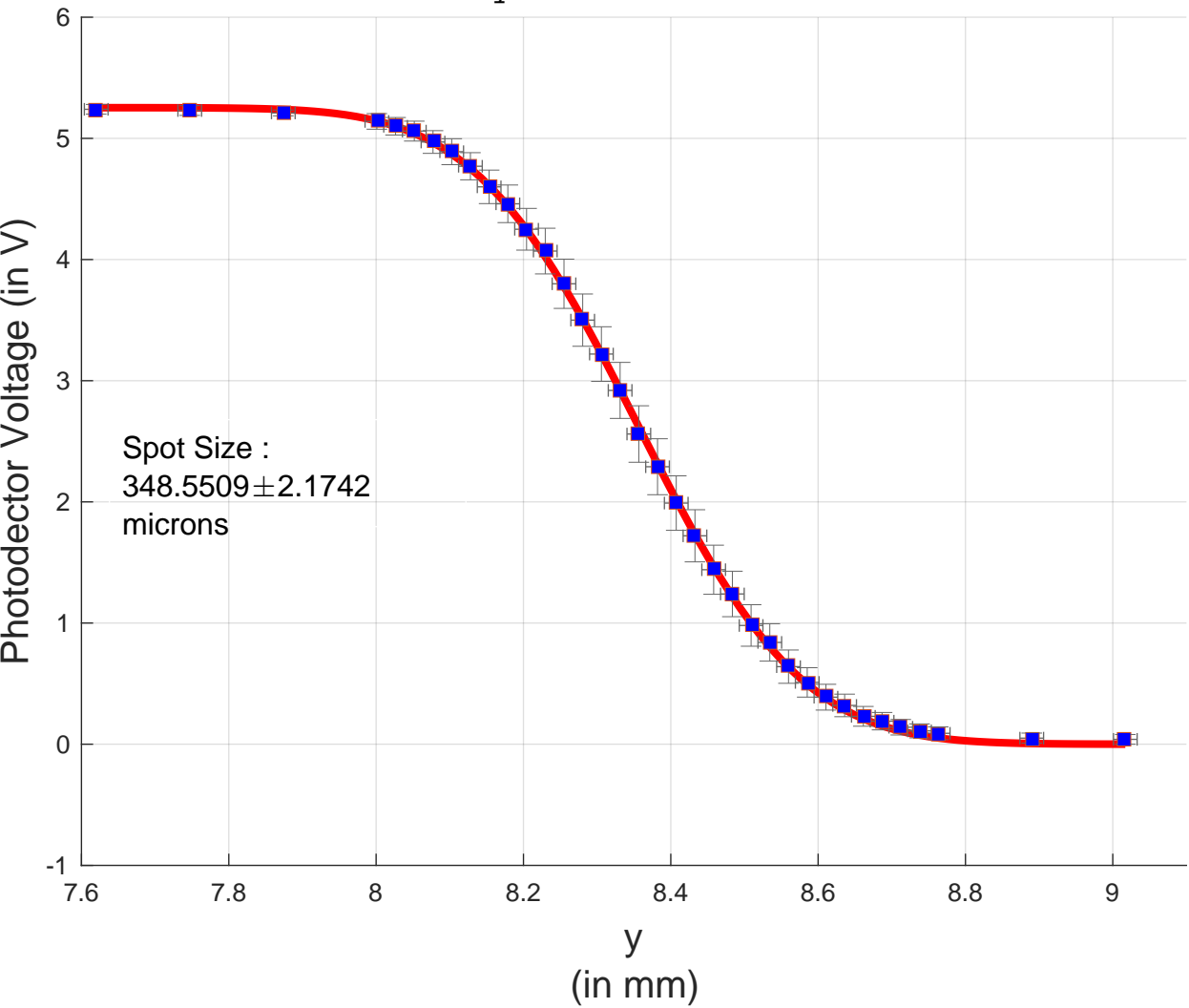
Beam y-Profile at z =15 cm
