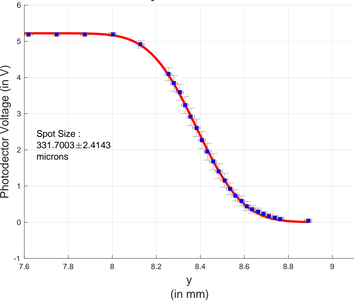
Beam y-Profile at z =4 cm
