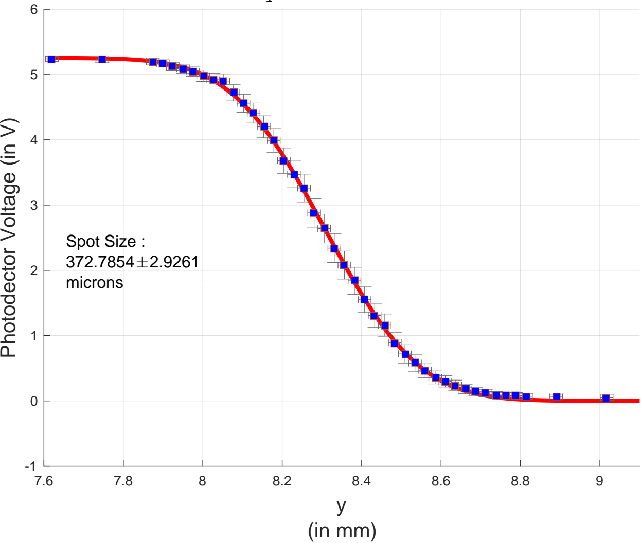
Beam y-Profile at z =25 cm
