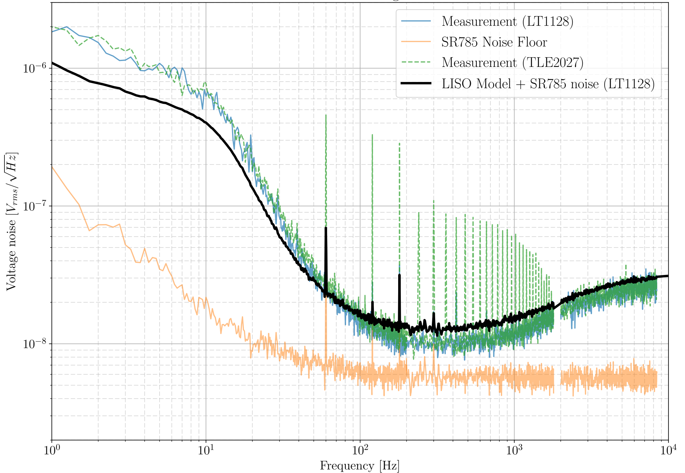
ITMX CH1 De-Whitening Board Noises
