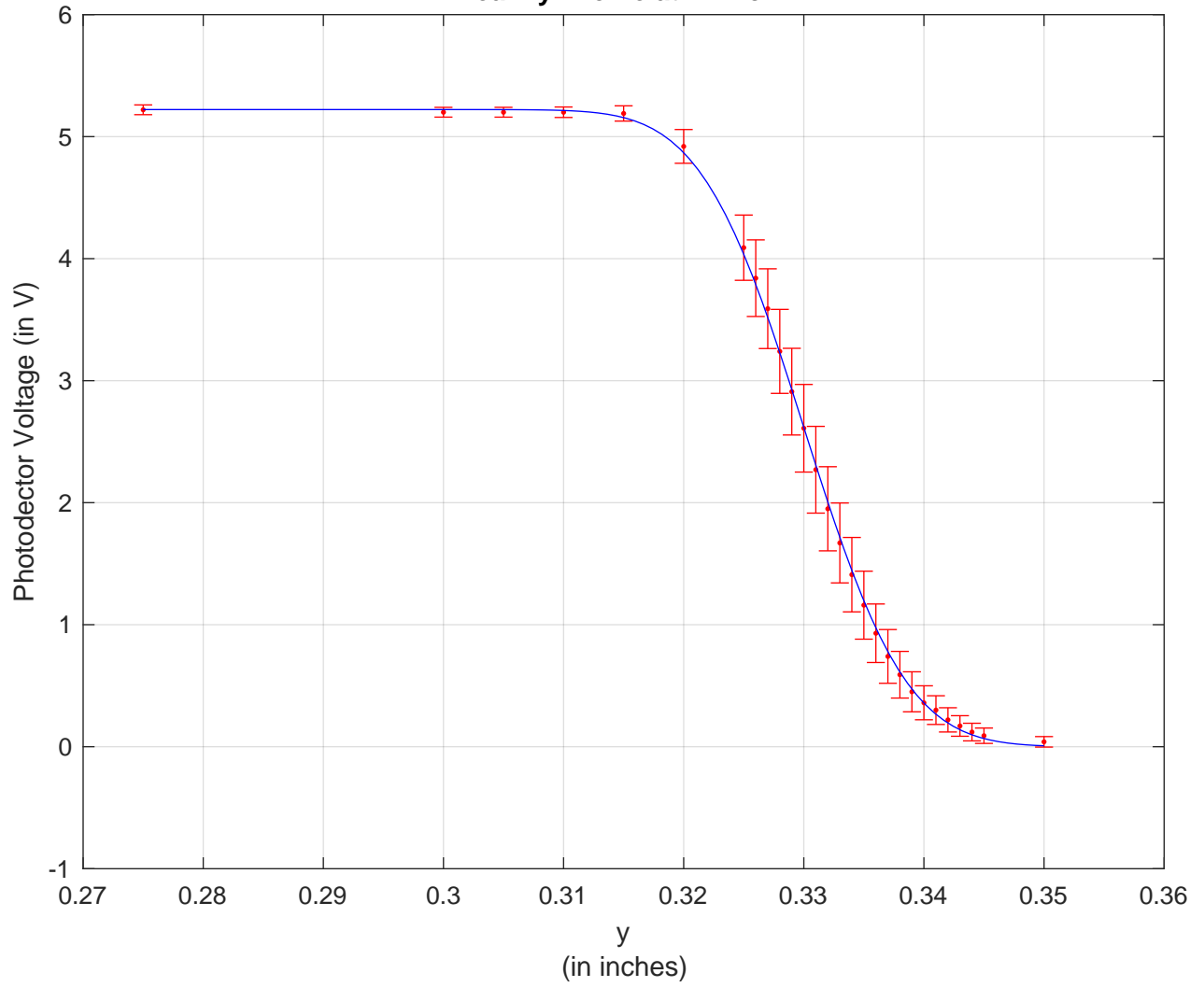
Beam y-Profile at z = 4cm
