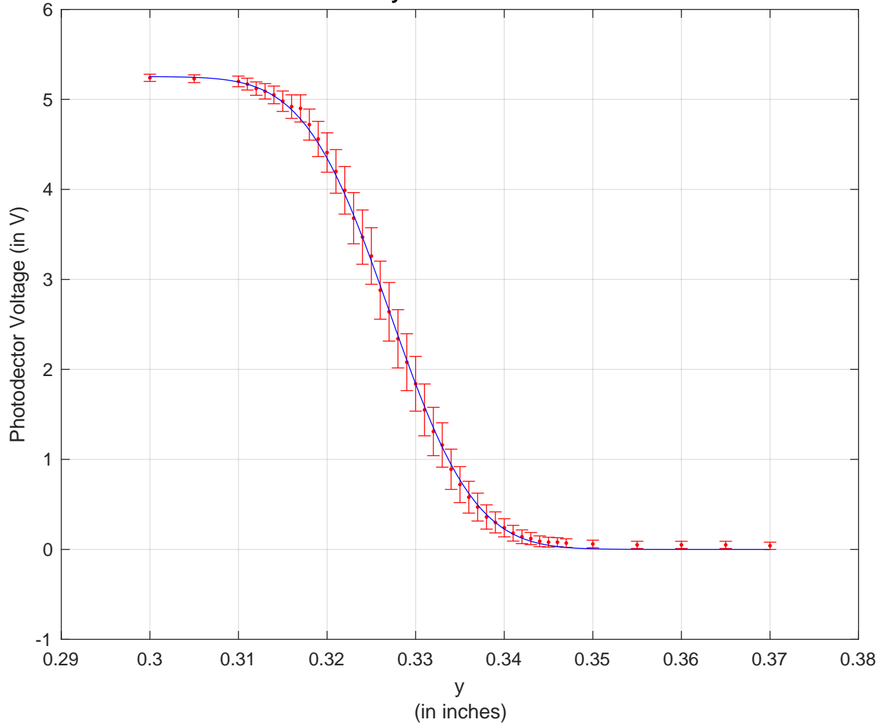
Beam y-Profile at z = 25cm
