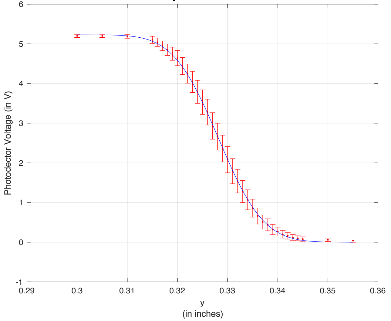
Beam y-Profile at z = 20cm
