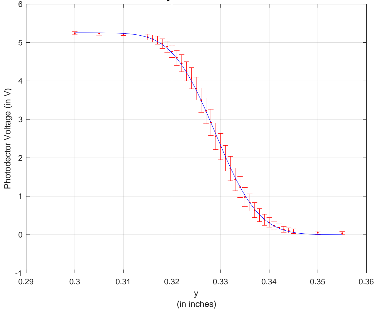
Beam y-Profile at z = 15cm
