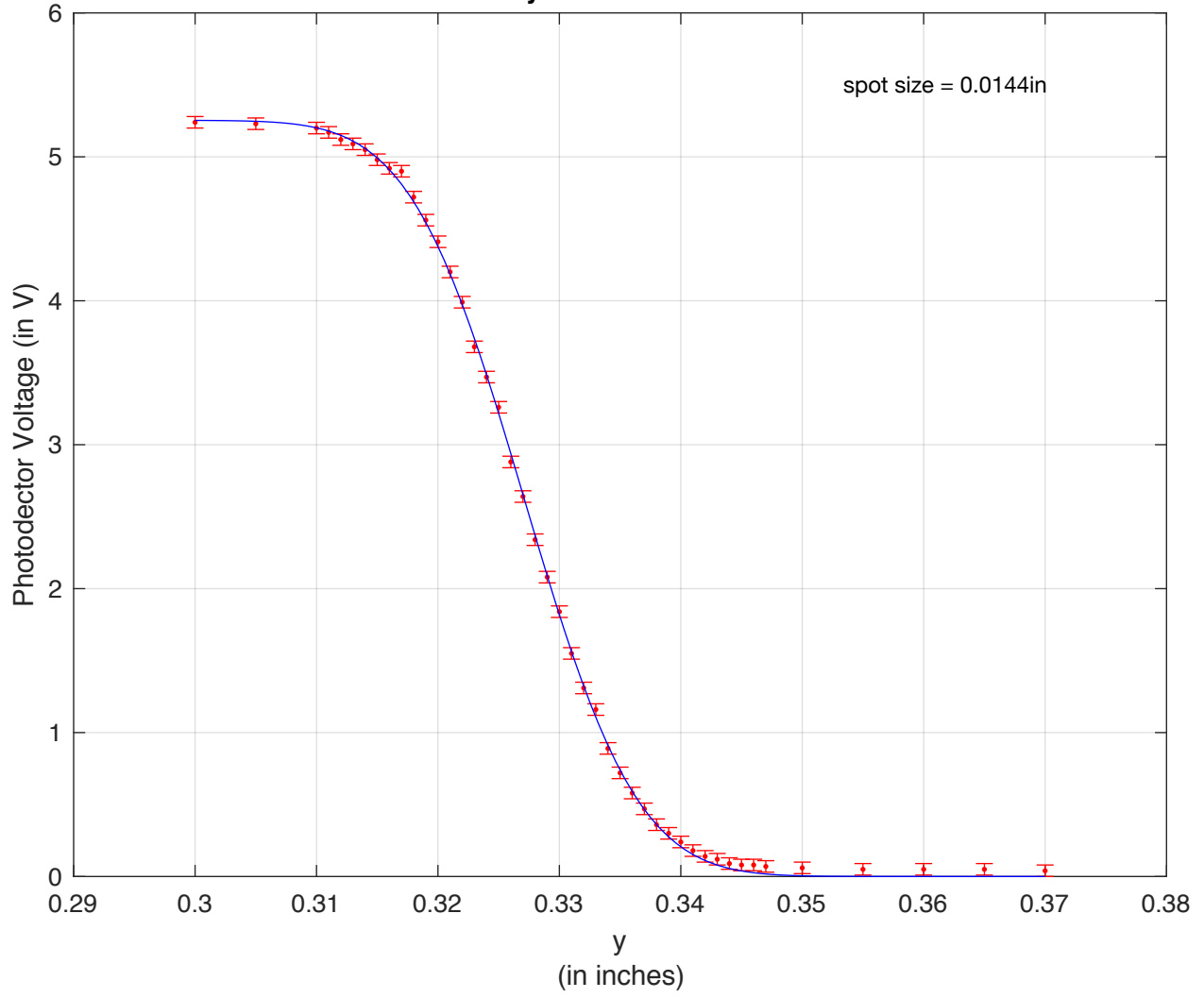
Beam y-Profile at z = 25cm
