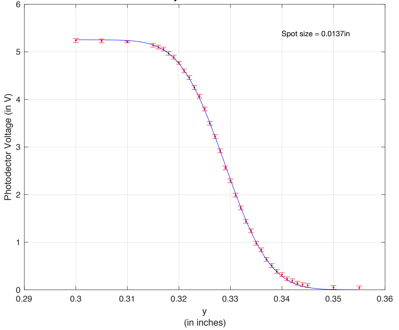
Beam y-Profile at z = 15cm
