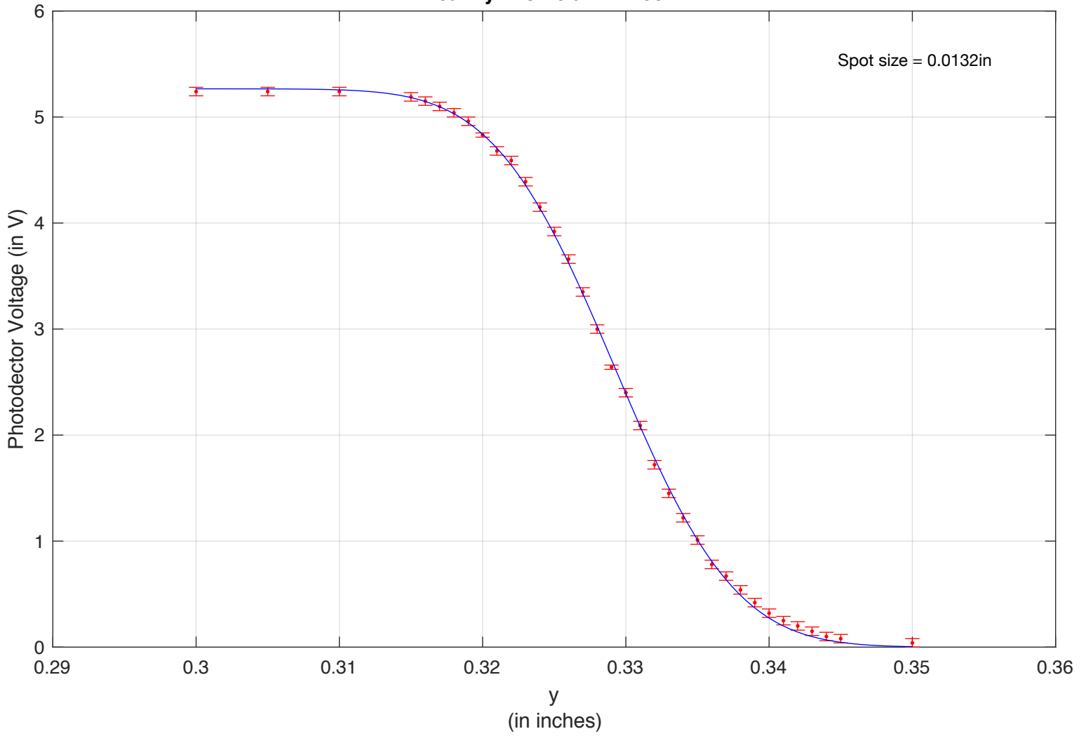
Beam y-Profile at z = 10cm
