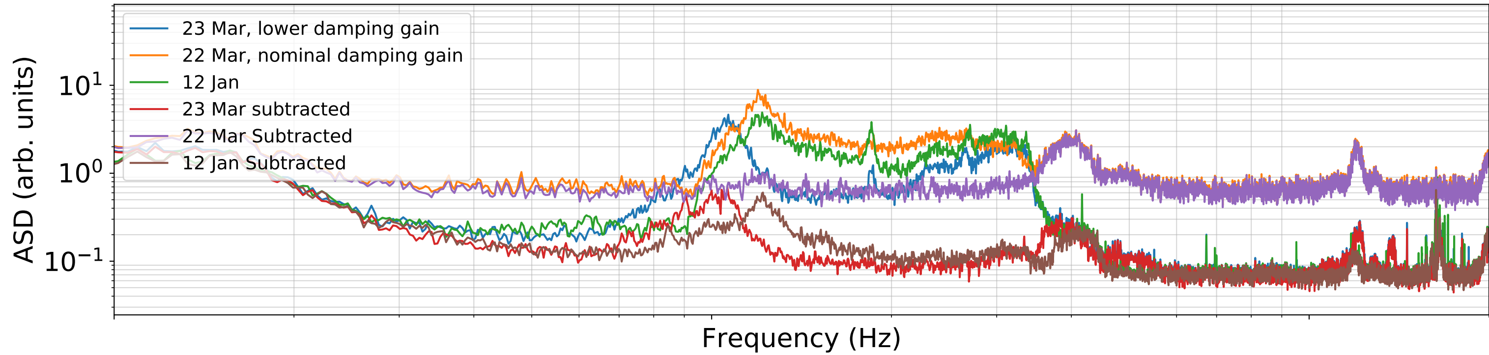
Multi-coherence between MCL and Seismometer channels
