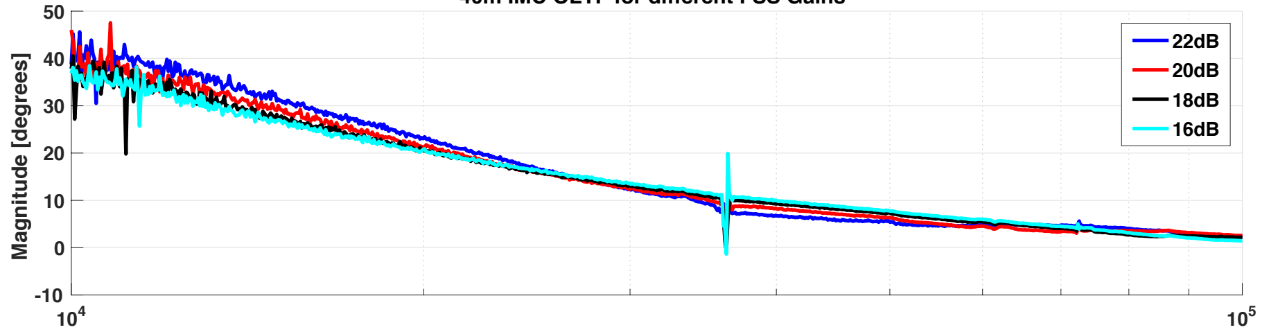
40m IMC OLTF for different FSS Gains
