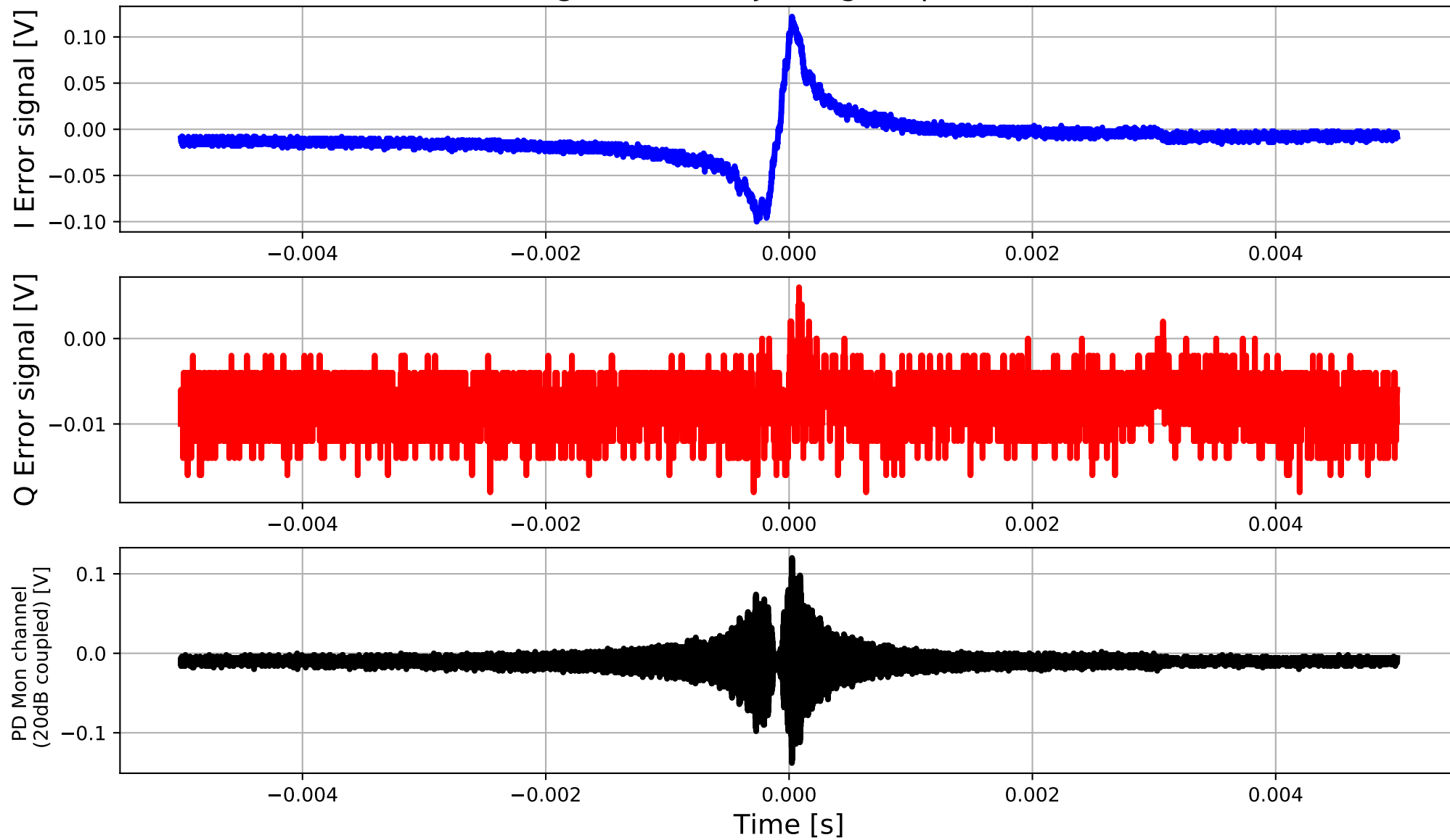
IMC PDH error signal after adjusting LO phase to Demod board
