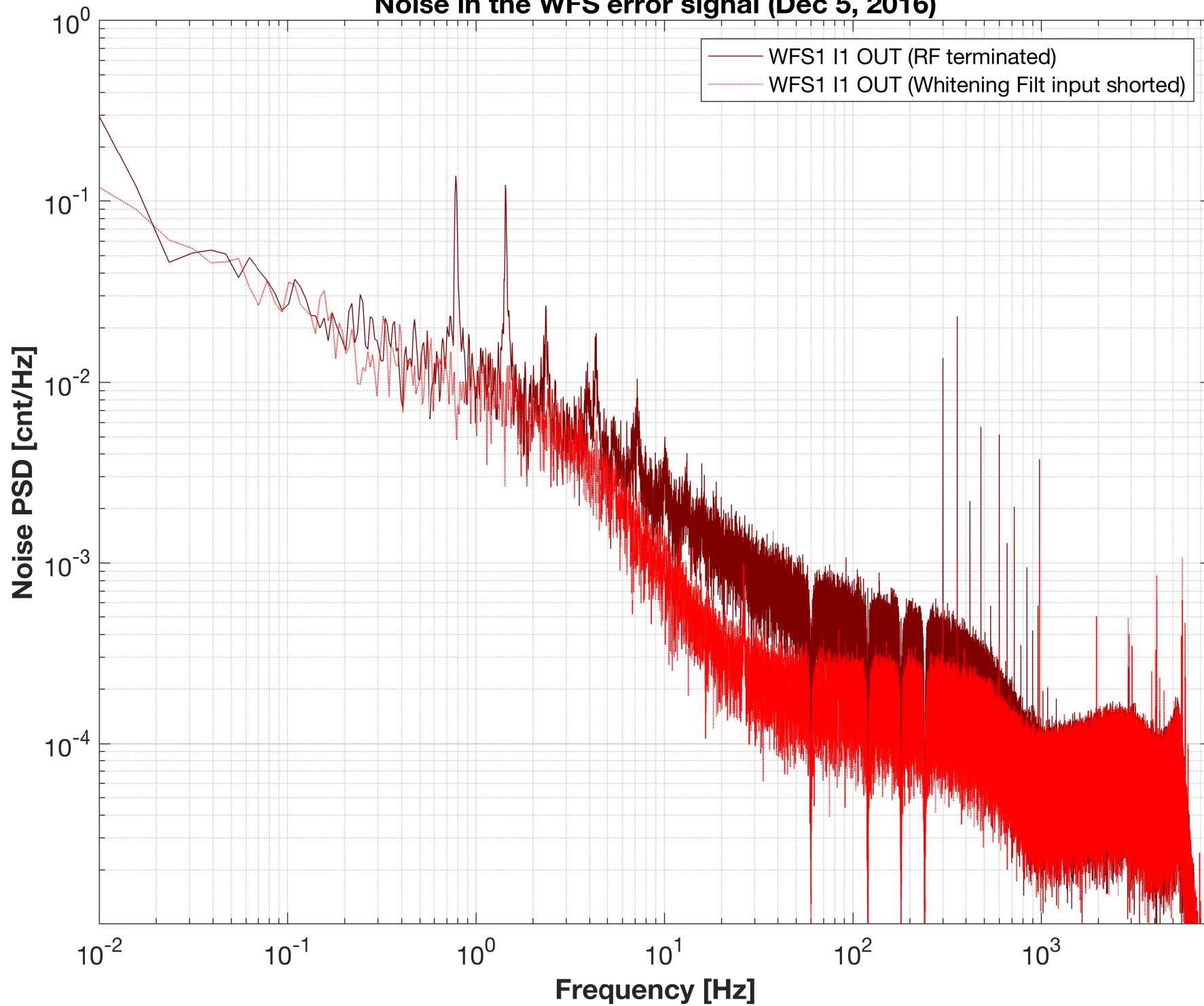
Noise in the WFS error signal (Dec 5, 2016)
