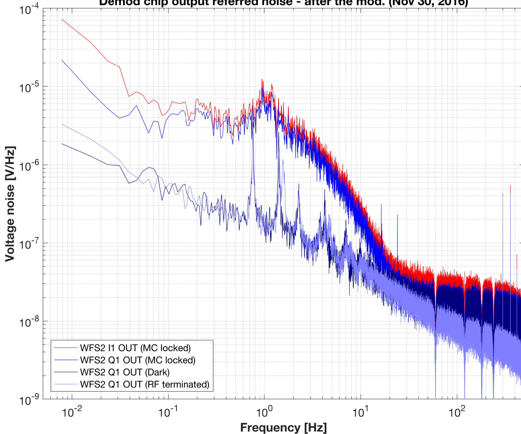
Demod chip output referred noise - after the mod. (Nov 30, 2016)
