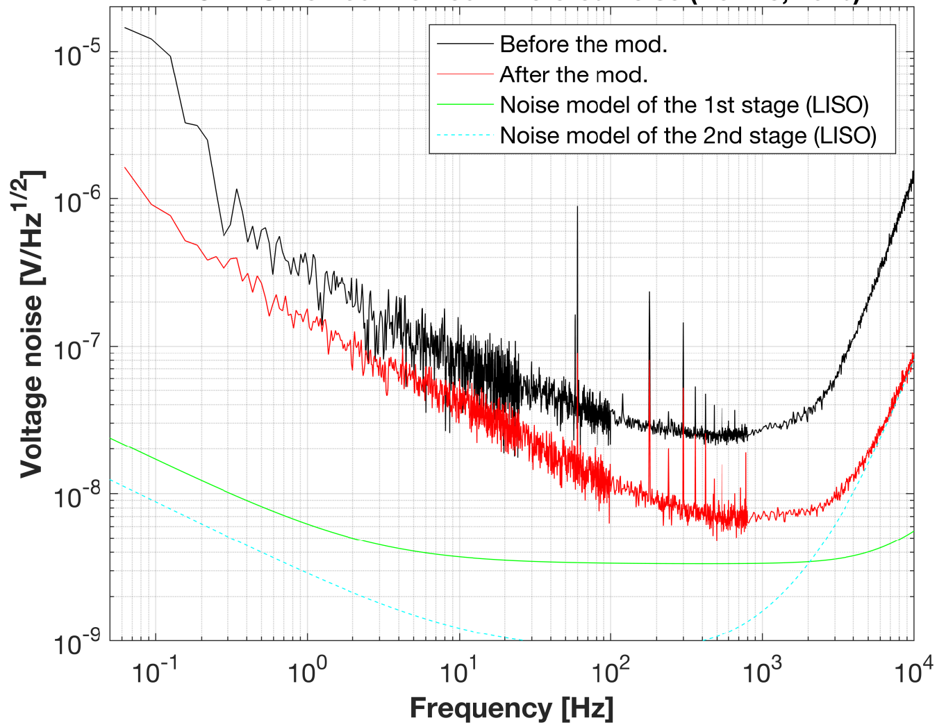
IMC WFS Demod: Demod-in refered noise (Nov 28, 2016)
