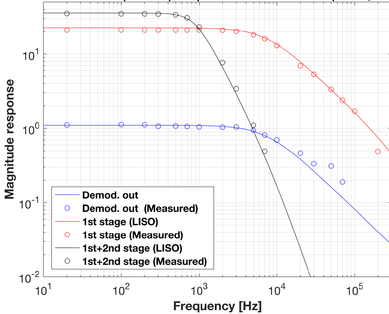
IMC WFS Demod (modified): Response ~ measured & model (Nov 28, 2016)
