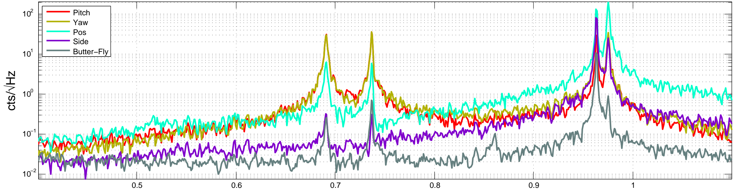
Calculated DOFs of ITMY before Input Matrix Diagonalization
