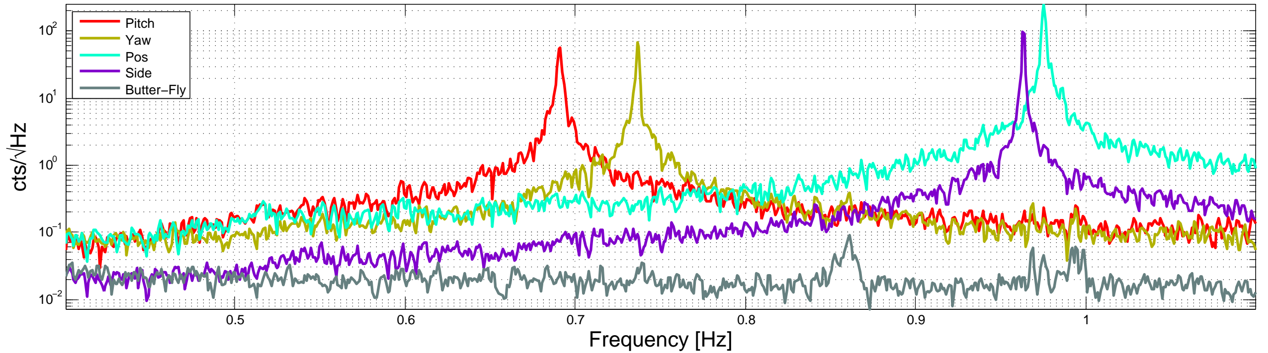
Calculated DOFs of ITMY after Input Matrix Diagonalization
